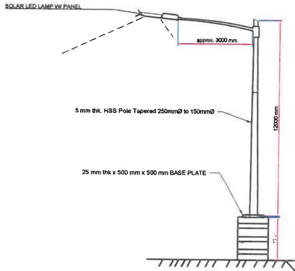
LAMP POST DETAIL SCALE NTS
