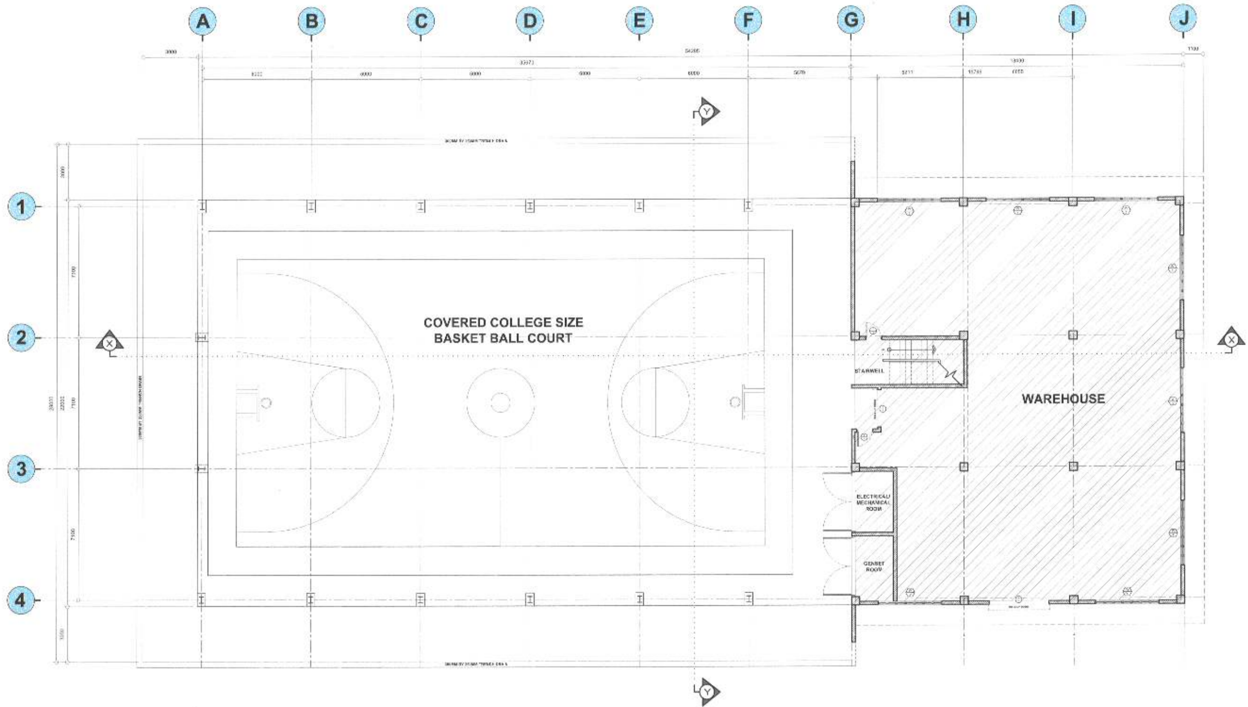
1 A 2 GROUND FLOOR PLAN SCALE 1:110 MTS.
