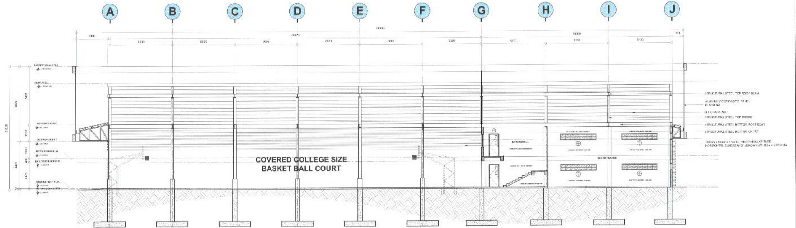
1 CROSS SECTION THRU "X" SCALE 1:115 MTS.
