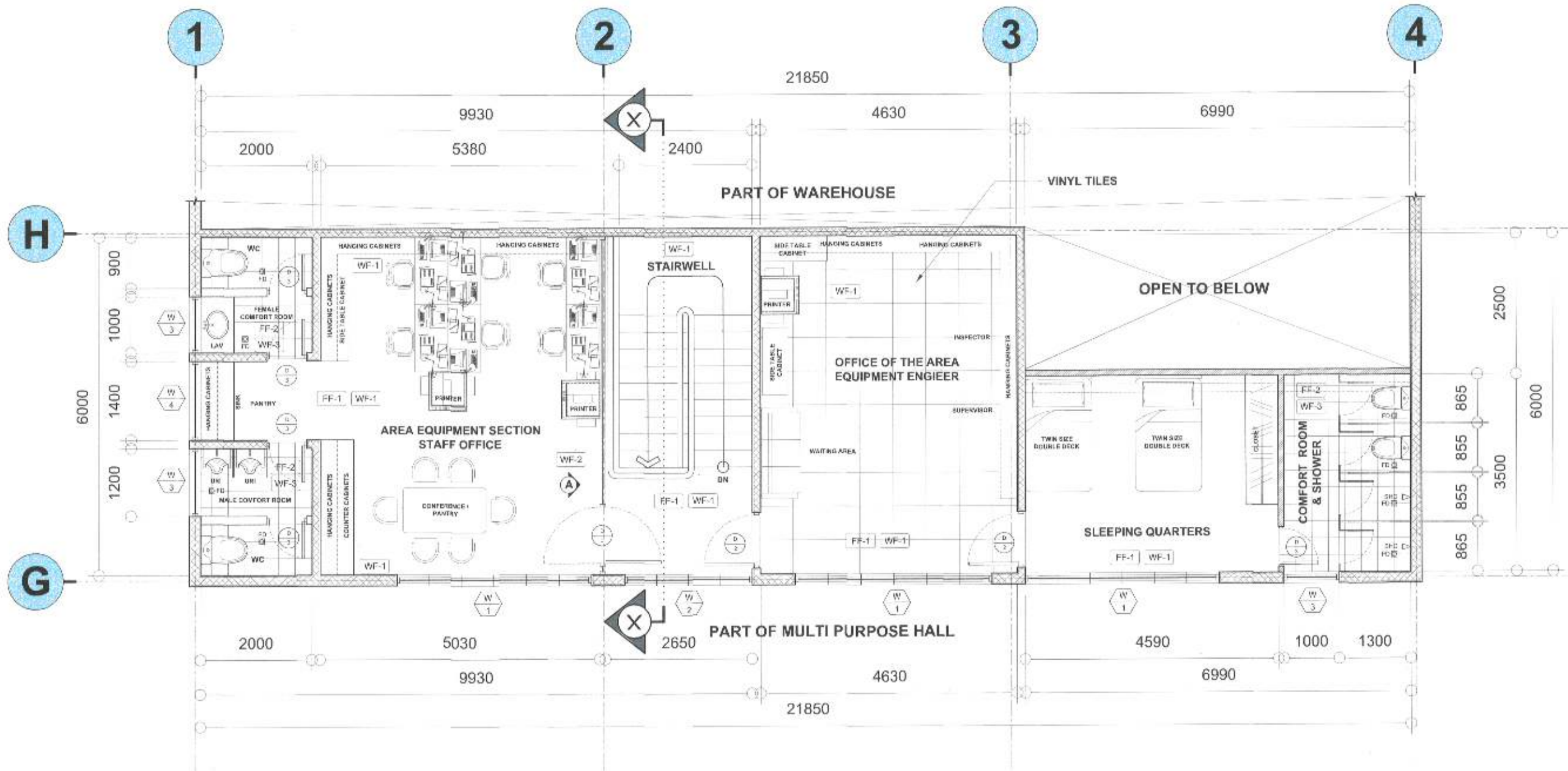
1 SECOND FLOOR PLAN (WAREHOUSE AREA) SCALE 1:45 MTS.
