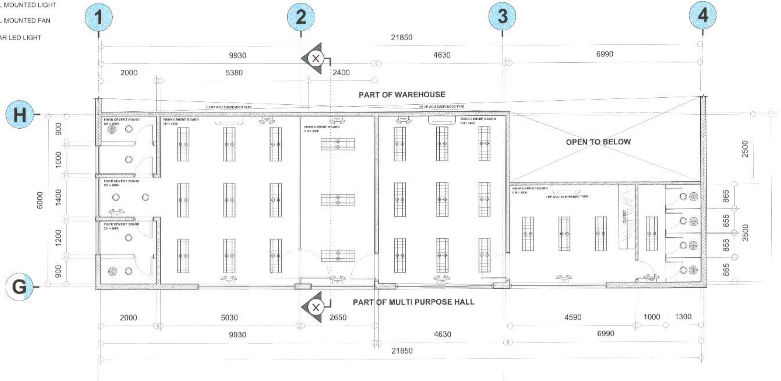
SECOND FLOOR REFLECTED CEILING PLAN (WAREHOUSE AREA)
