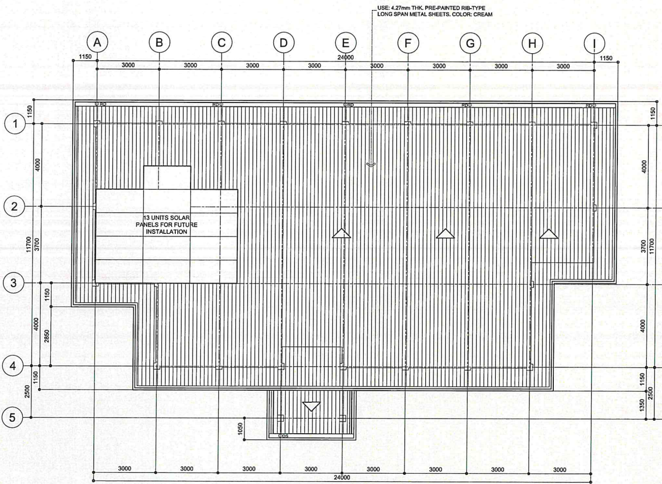
1 TYPICAL ROOF PLAN (UNIT 1 & 2) A-2 SCALE 1:100 M
