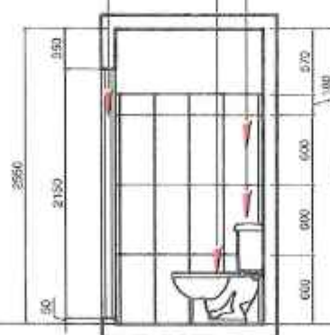
ELEVATION D SCALE: 1:40 METERS
