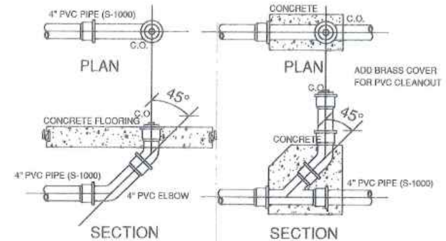
FLOOR CLEAN OUT DETAILS SCALE: NTS
