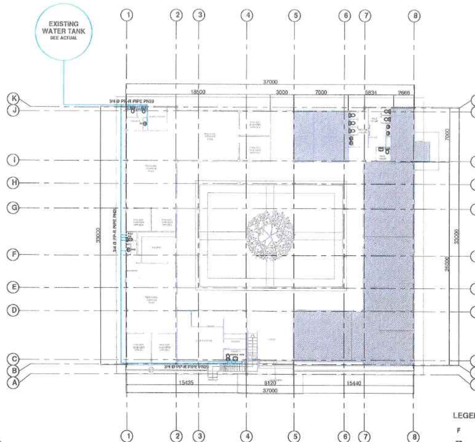
5 WATERLINE LAYOUT SCALE: 1:200 METERS
