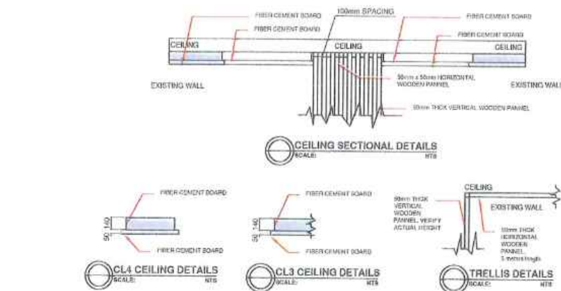
11 CEILING DETAILS AT CHIEF'S OFFICE A 6 SCALE: NTS
