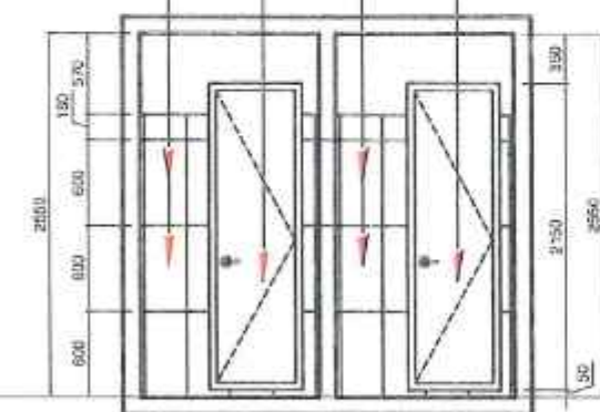
ELEVATION C SCALE: 1:40 METERS
