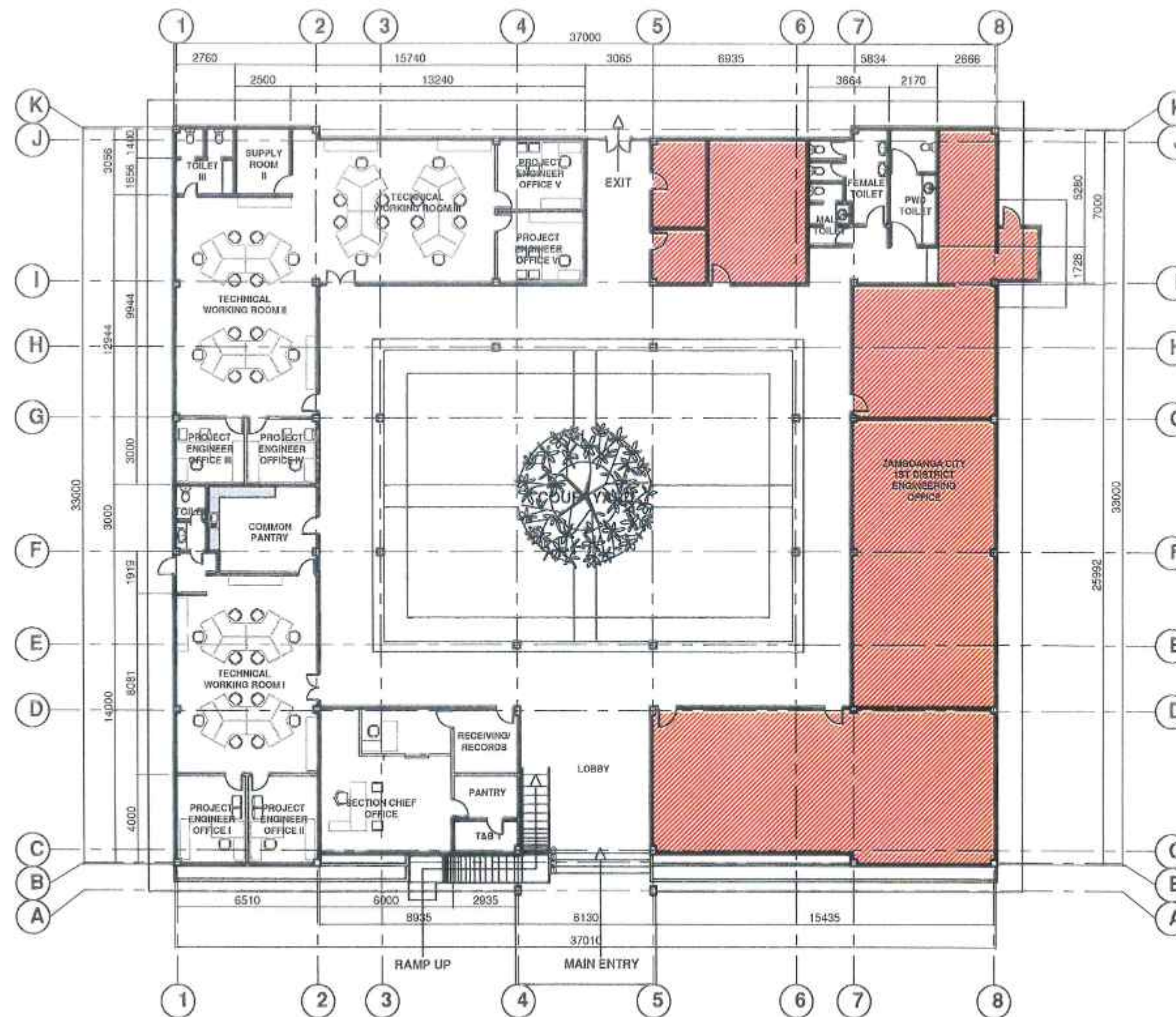
4 EXISTING FLOOR PLAN SCALE: 1:150 METERS
