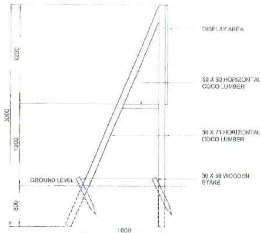
TYPICAL FRAME ELEVATION
