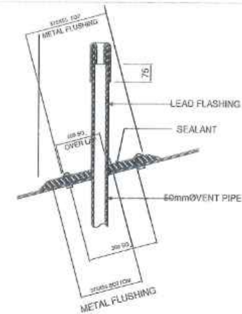
VENT THRU ROOF DETAIL SCALE: NTS
