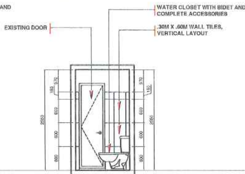
ELEVATION B SCALE: 1:40 METERS
