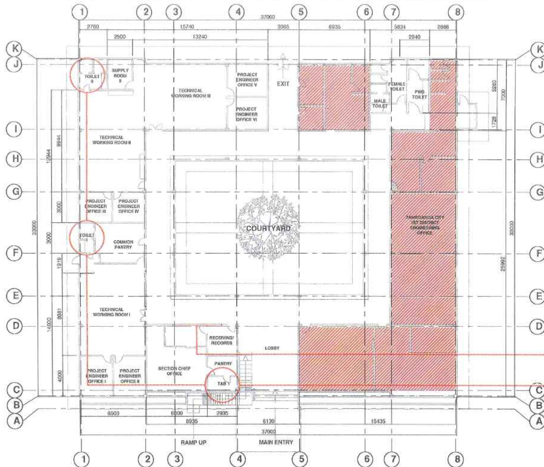
5 DEMOLITION PLAN A 3 SCALE: 1:200 METERS
