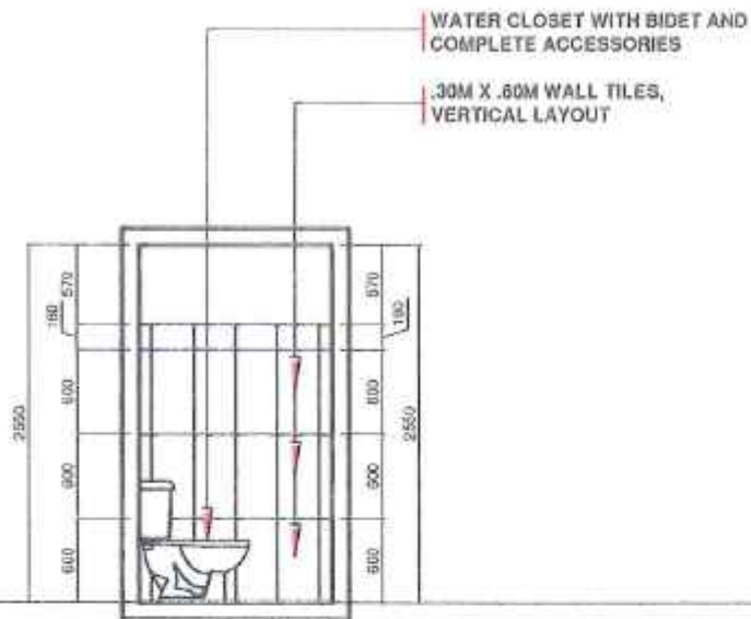
ELEVATION A SCALE: 1:40 METERS
