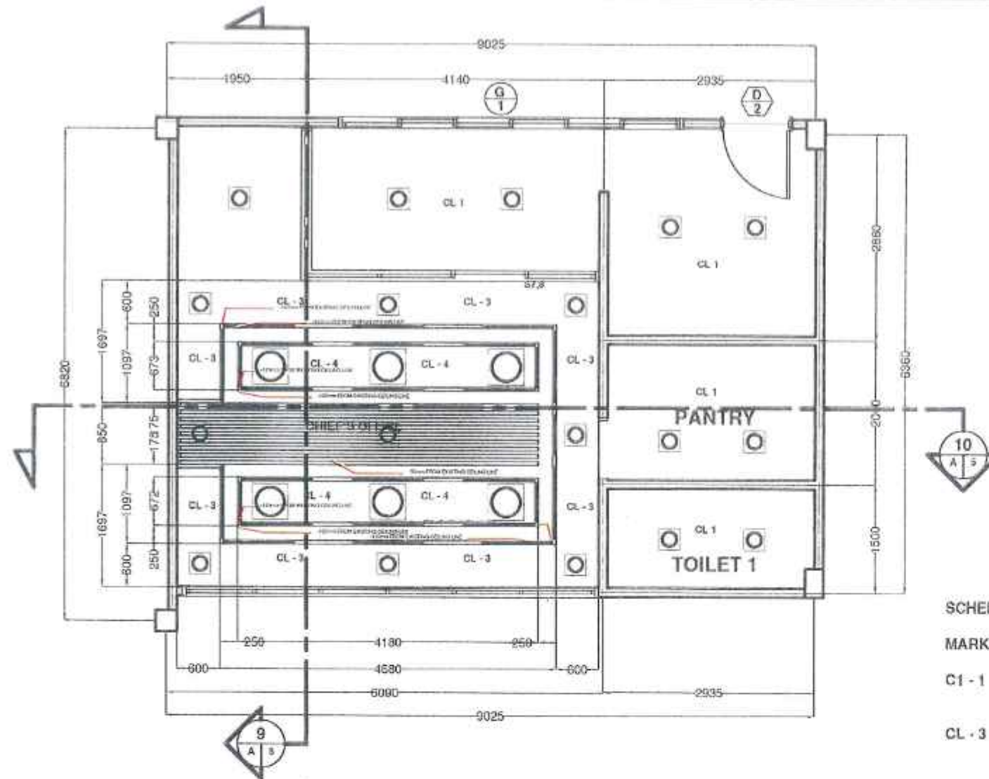
7 REFLECTED CEILING PLAN AT CHIEF'S OFFICE SCALE: 1:50 METERS
