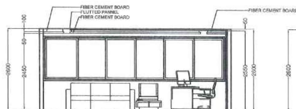
9 SECTION THRU X - X' SCALE: 1:50 METERS
