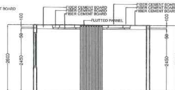
10 SECTION THRU Y - Y' SCALE: 1:50 METERS
