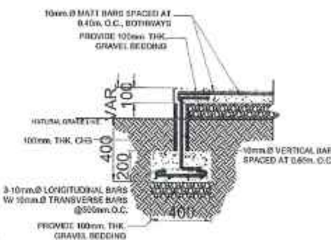
WALL FOOTING SECTION DETAIL
