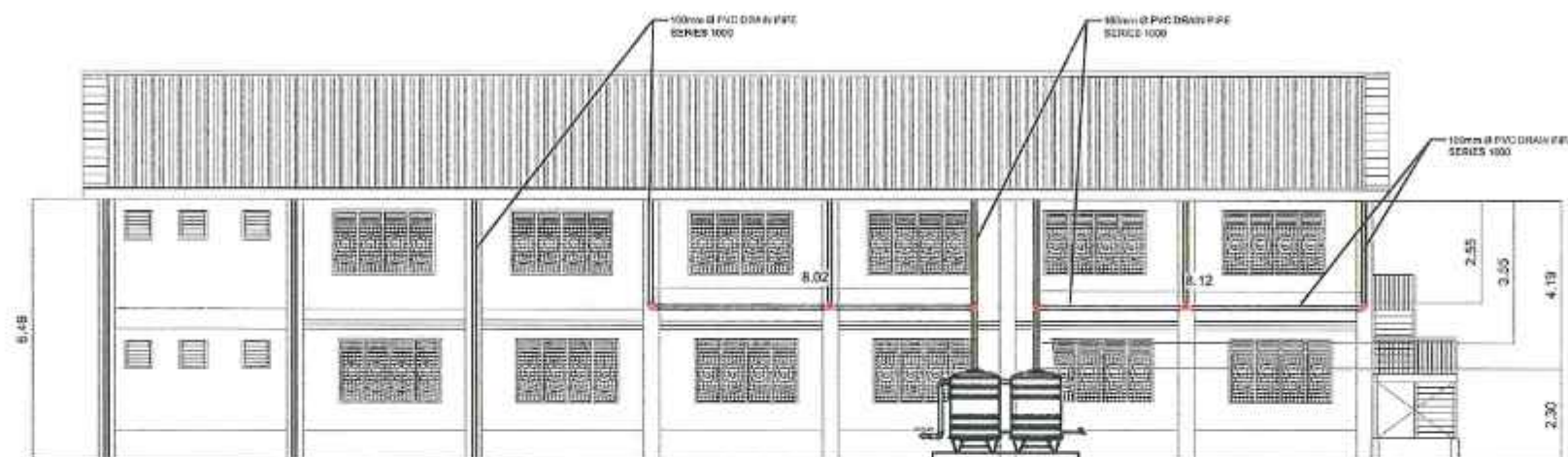
REAR ELEVATION SCALE 1:100 M.
