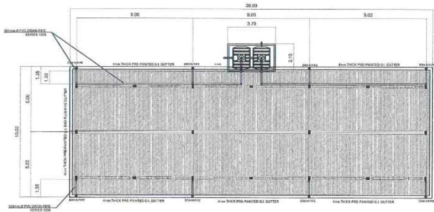
1 STOREY - 3 CLASSROOM SCHOOL BUILDING ROOF PLAN SCALE 1:100 M.
