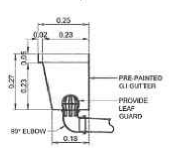
GUTTER BLOW-UP DETAIL
