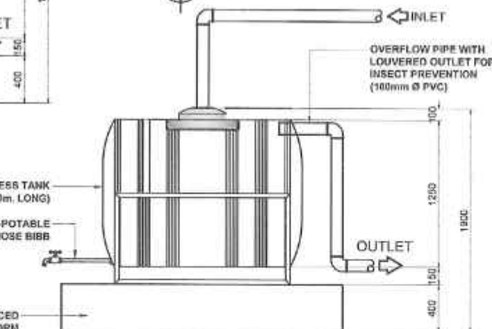
RIGHT-SIDE ELEVATION
