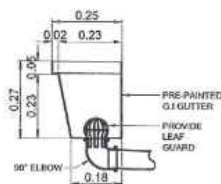
GUTTER BLOW-UP DETAIL
