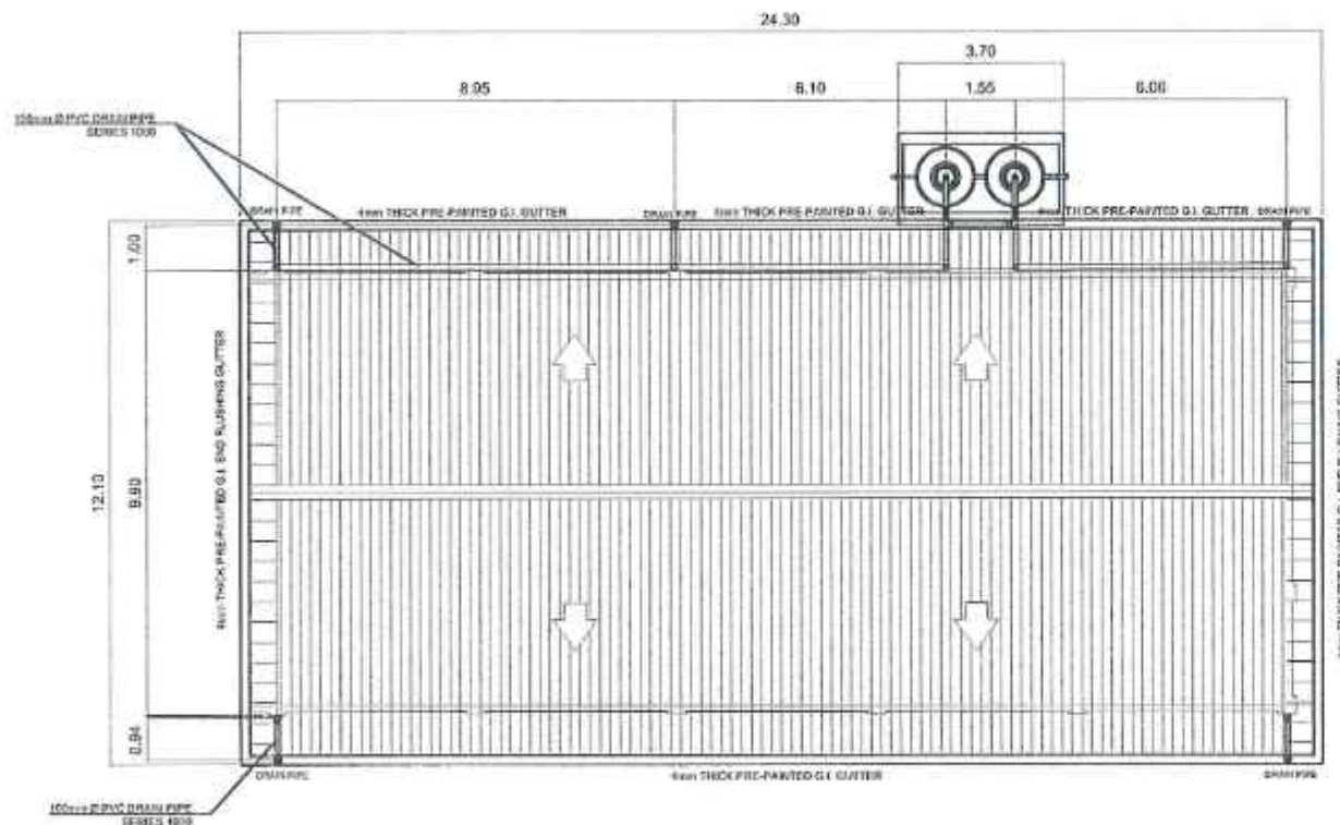
2 STOREY - 4 CLASSROOM SCHOOL BUILDING ROOF PLAN
