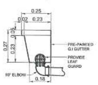
GUTTER BLOW-UP DETAIL
