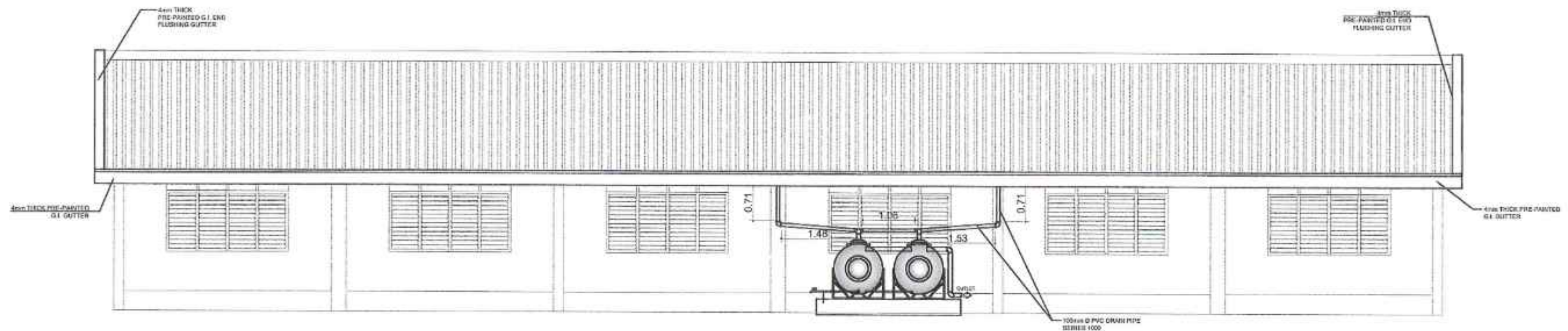
REAR ELEVATION SCALE 1:50 M.
