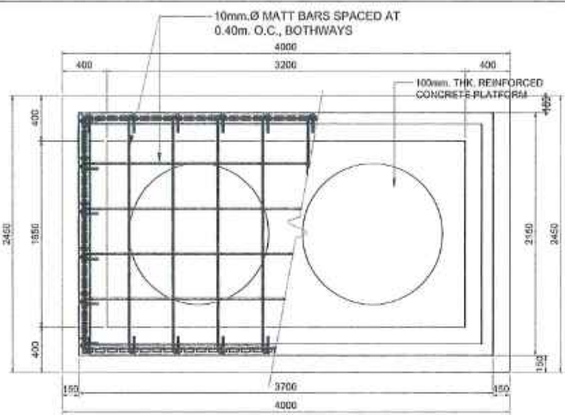
FOUNDATION PLAN
