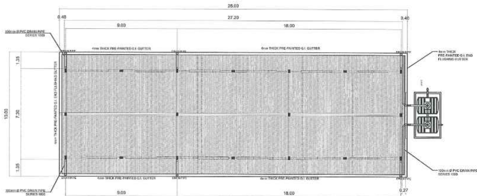
1 STOREY - 3 CLASSROOM SCHOOL BUILDING ROOF PLAN
