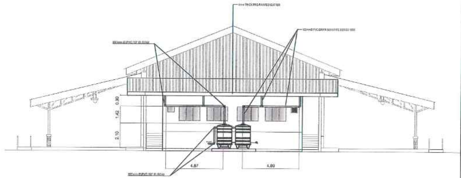
REAR ELEVATION
