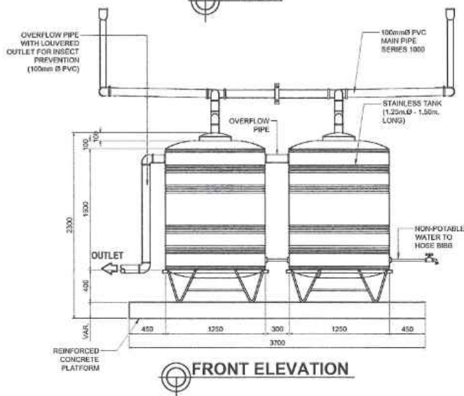
RAIN WATER COLLECTION SYSTEM DETAIL
