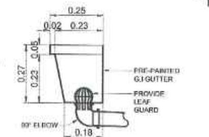
GUTTER BLOW-UP DETAIL
