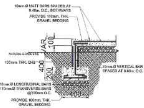
WALL FOOTING SECTION DETAIL
