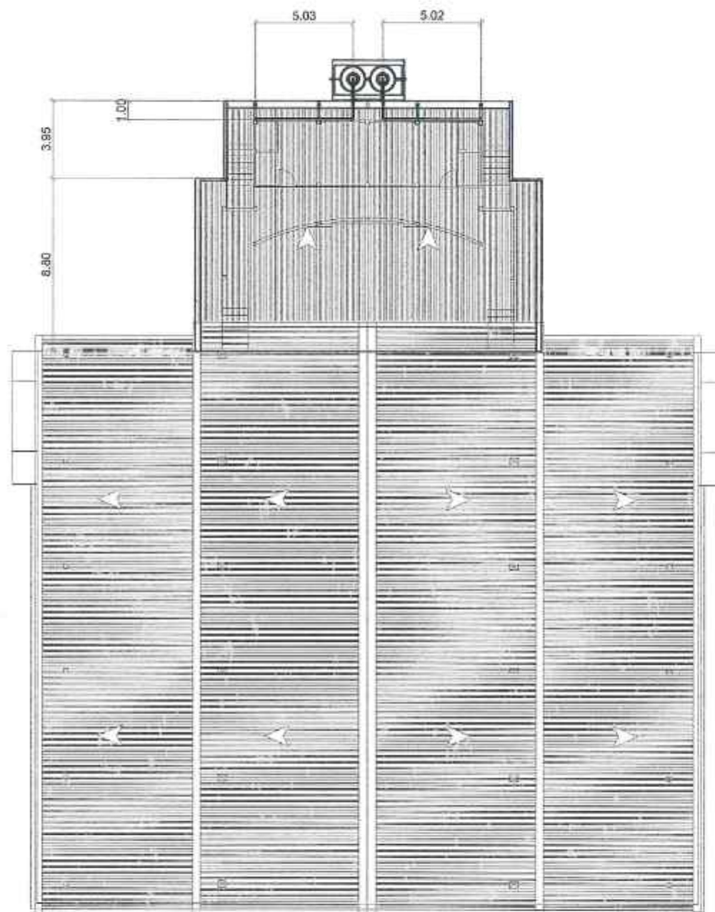
COVERED COURT - TUMITUS ROOF PLAN
