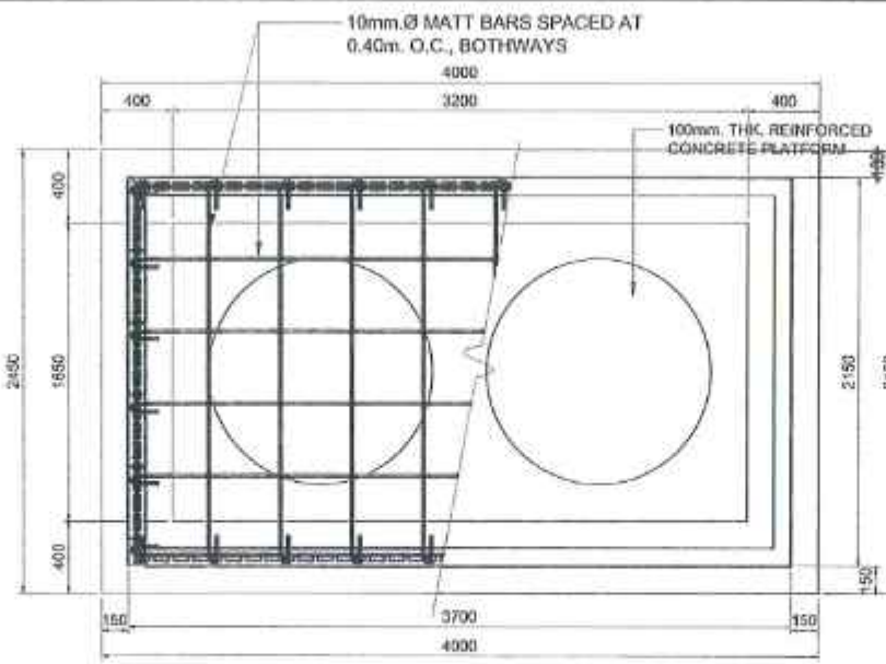
FOUNDATION PLAN
