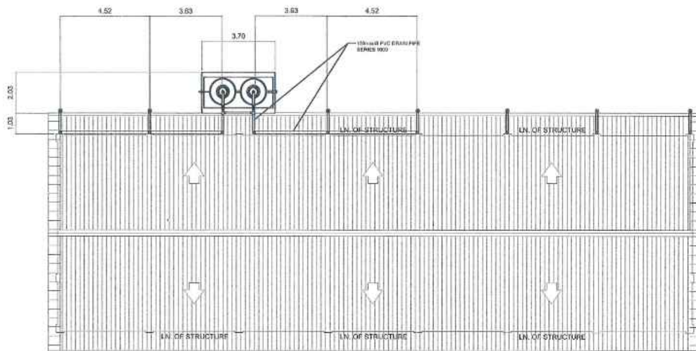
2 STOREY - 4 CLASSROOM SCHOOL BUILDING ROOF PLAN
