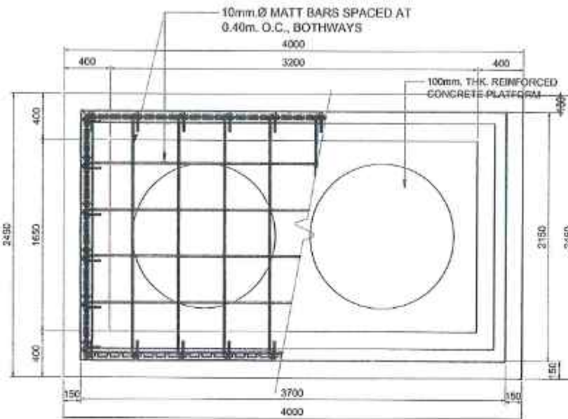
FOUNDATION PLAN
