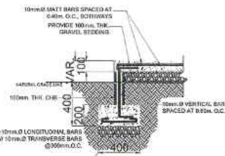
WALL FOOTING SECTION DETAIL
