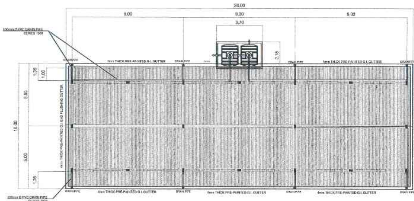
1 STOREY - 3 CLASSROOM SCHOOL BUILDING ROOF PLAN
