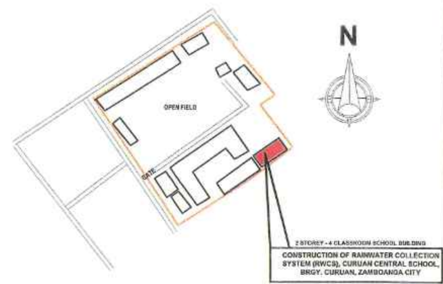
SITE DEVELOPMENT PLAN
