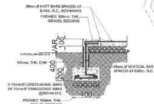
WALL FOOTING SECTION DETAIL
