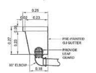
GUTTER BLOW-UP DETAIL SCALE: 1:10 MTRS.
