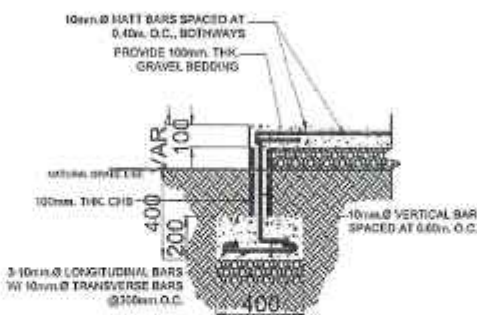
WALL FOOTING SECTION DETAIL
