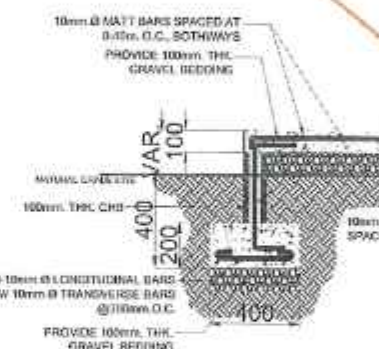
WALL FOOTING SECTION DETAIL
