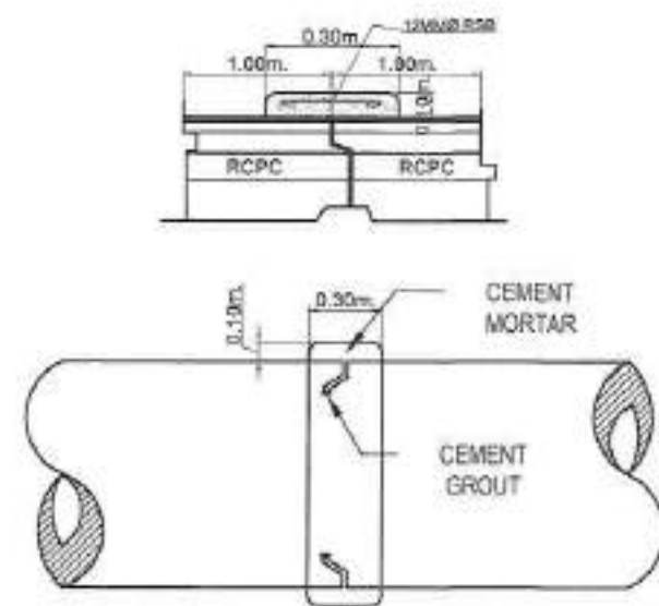
3B PIPE COLLAR DETAIL SCALE NTS
