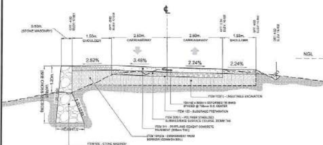
01 TYPICAL ROAD SECTION DETAIL 'A' SCALE 1:60
