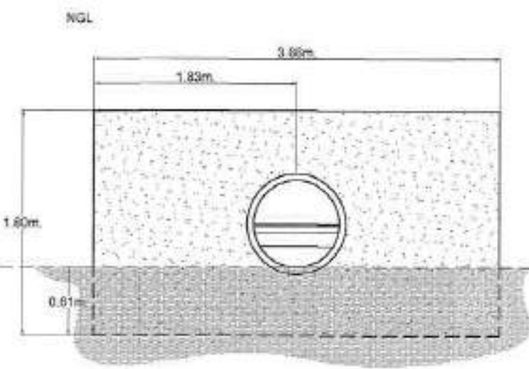
3A LEFT AND RIGHT HEADWALL DETAIL SCALE 1:20
