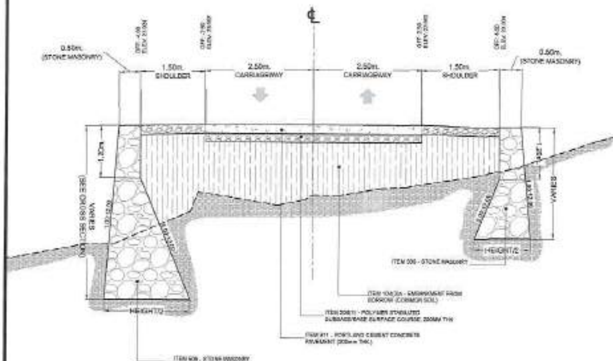
02 TYPICAL ROAD SECTION DETAIL 'B' SCALE 1:60
