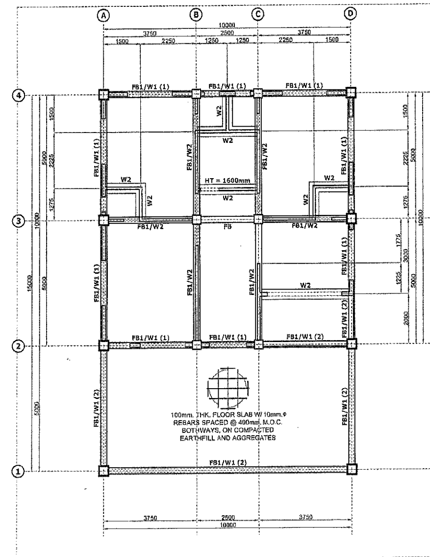
2 FLOOR FRAMING PLAN S-1 SCALE: 1:70 MTS.
