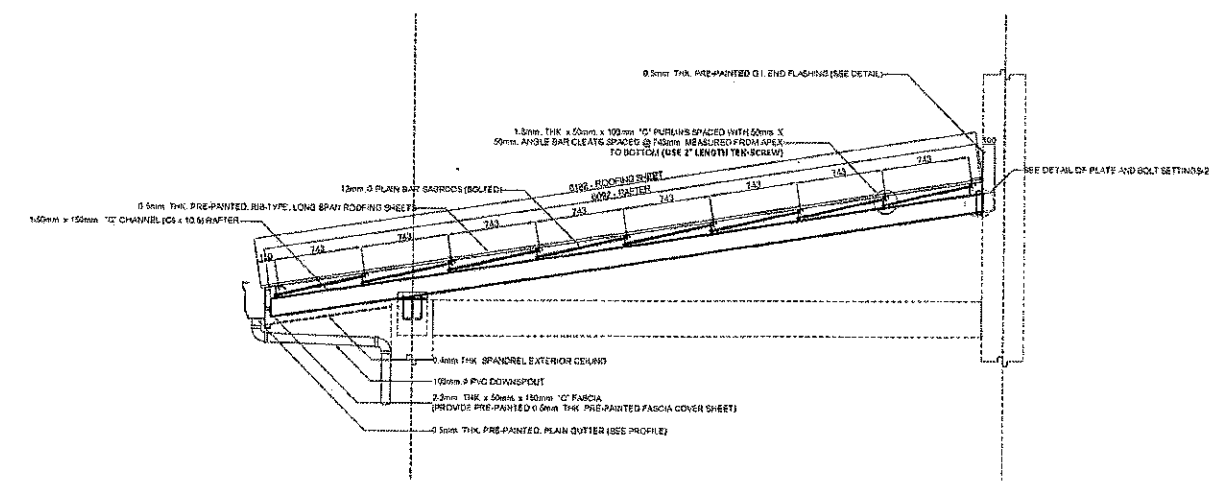
3 DETAILS OF RAFTER - 2 S-3 SCALE: 1:30 MTS.
