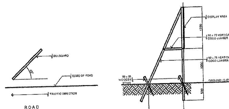
TYPICAL FRAME ELEVATION
