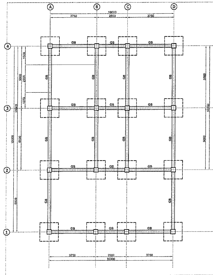
1 FOUNDATION PLAN S-1 SCALE: 1:70 MTS.
