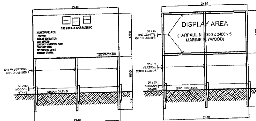
REAR ELEVATION
