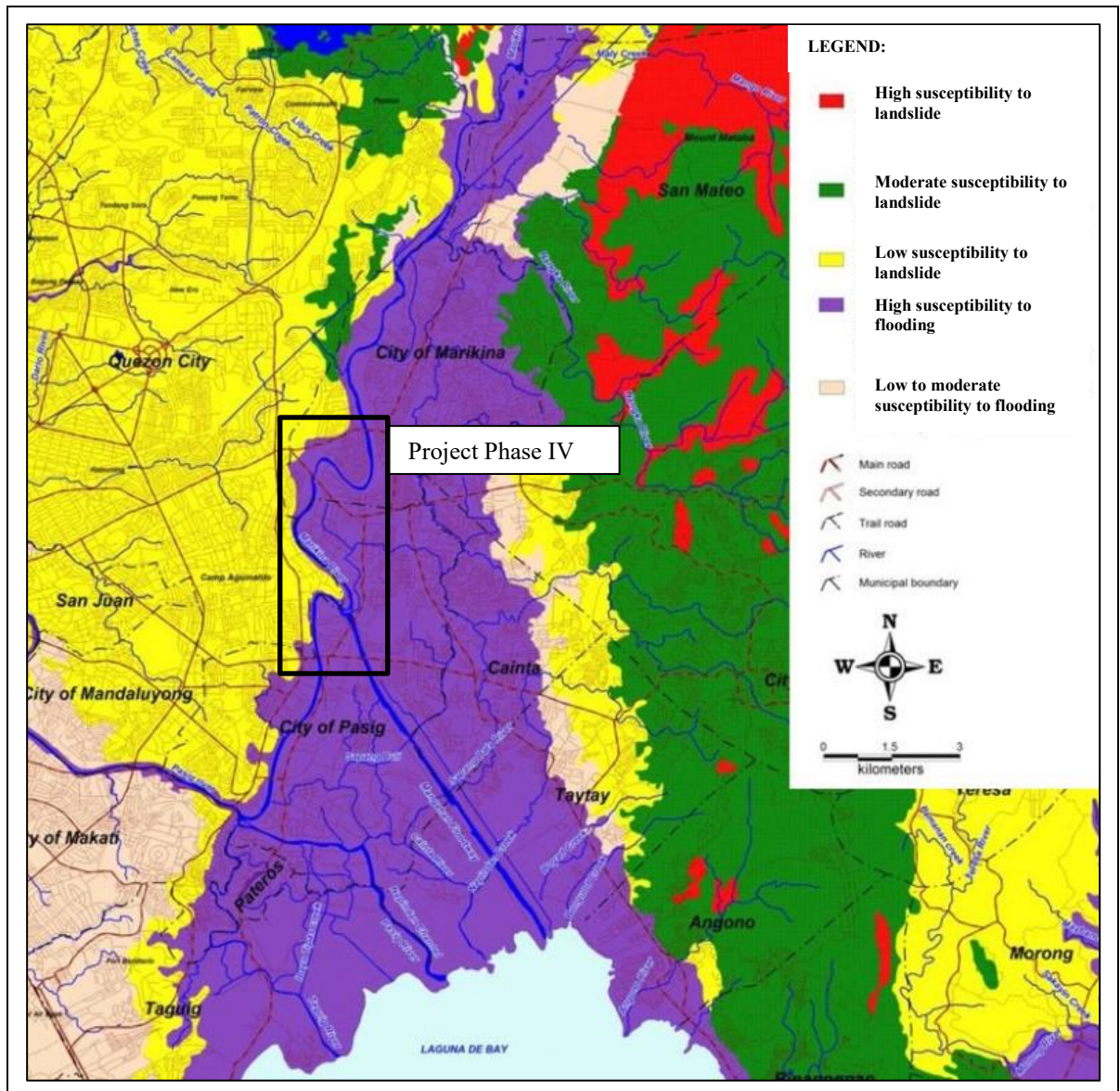
Figure 6.3.8 Flooding and Landslide Hazard Map of Metro Manila and Nearby Areas
