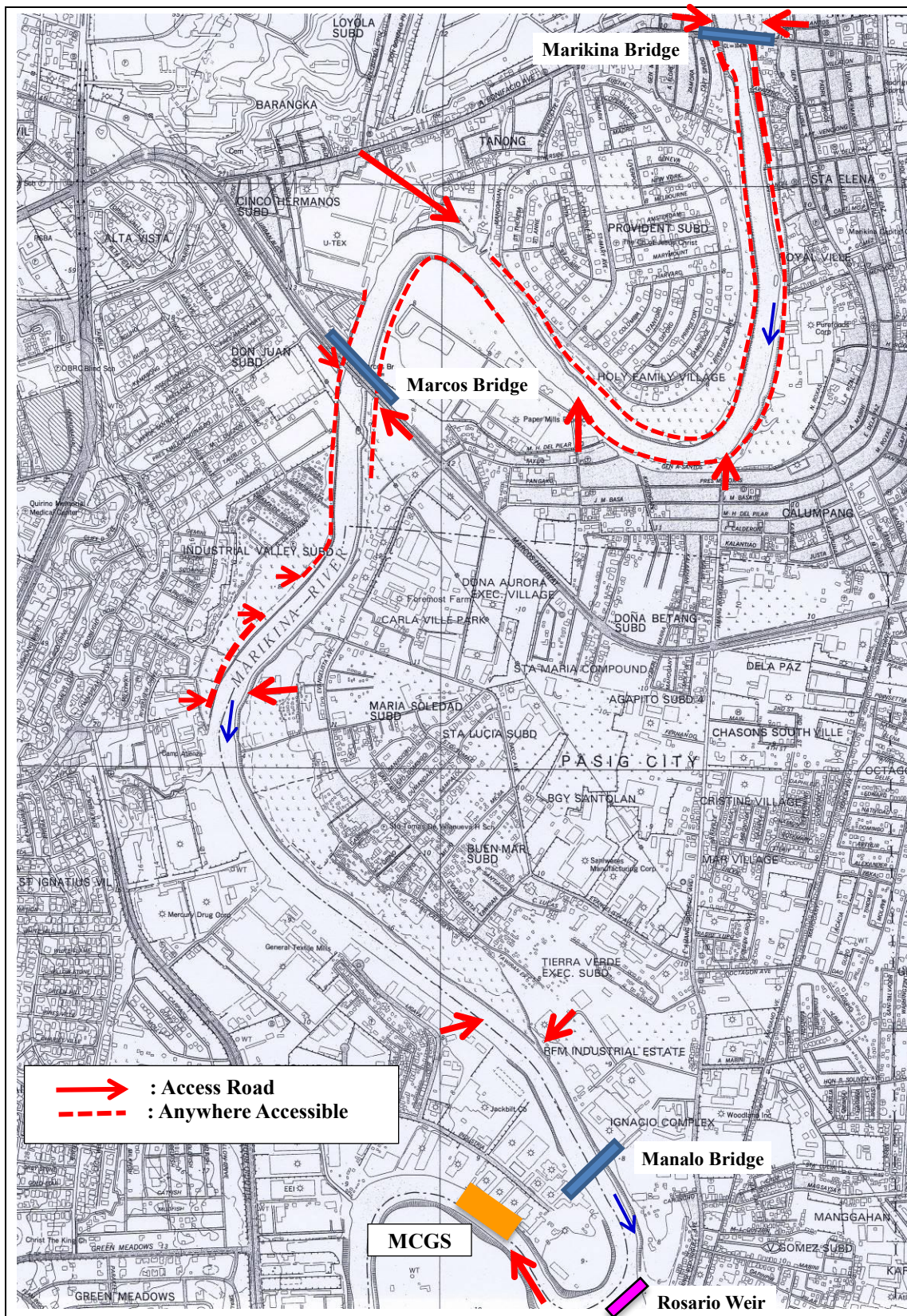
Figure 2.4.1 Candidate Location of Access Roads to Construction Sites
