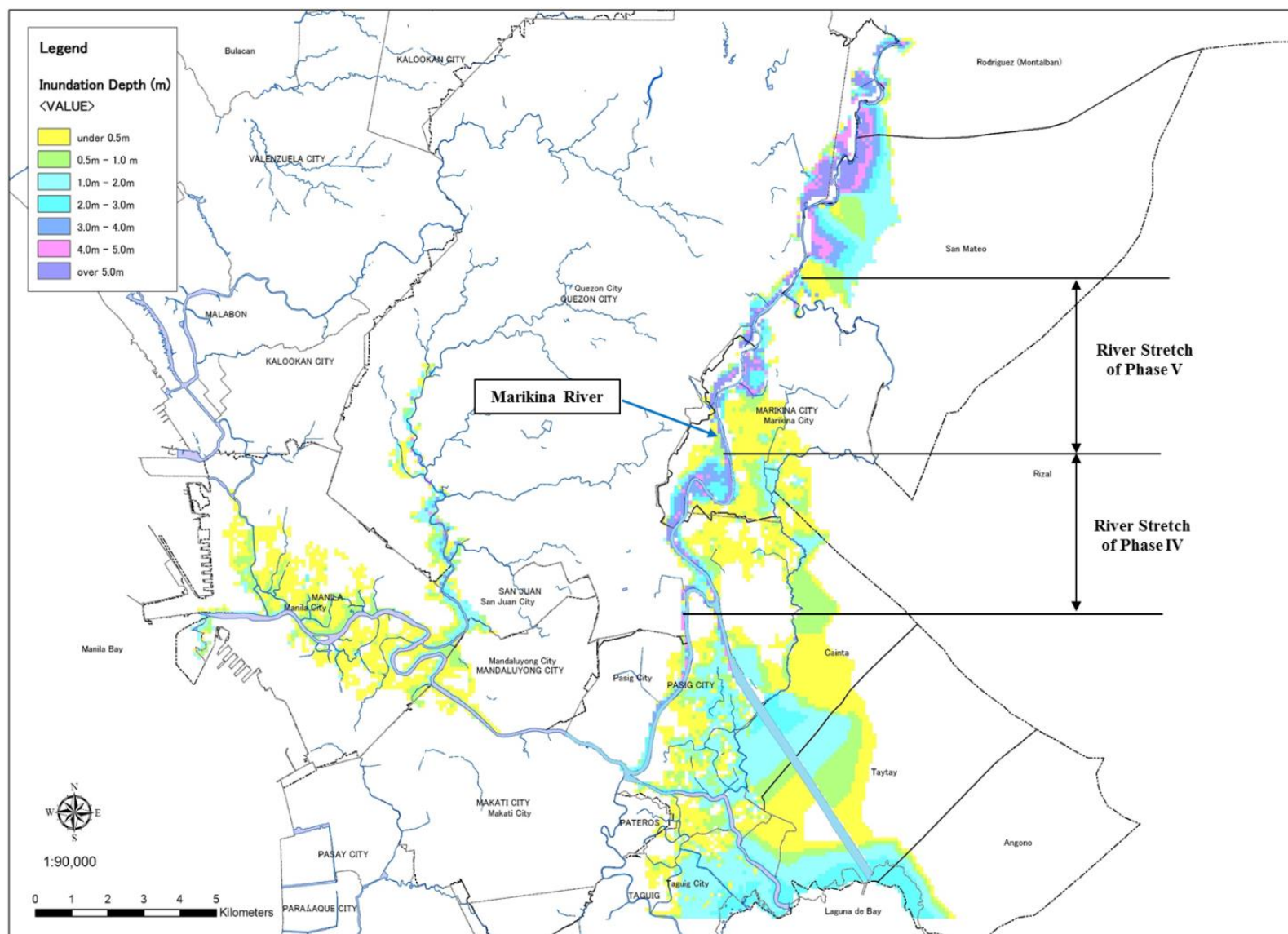
Figure 6.3.10 Inundation Area due to Tropical Storm Ondoy, Sep. 2009
