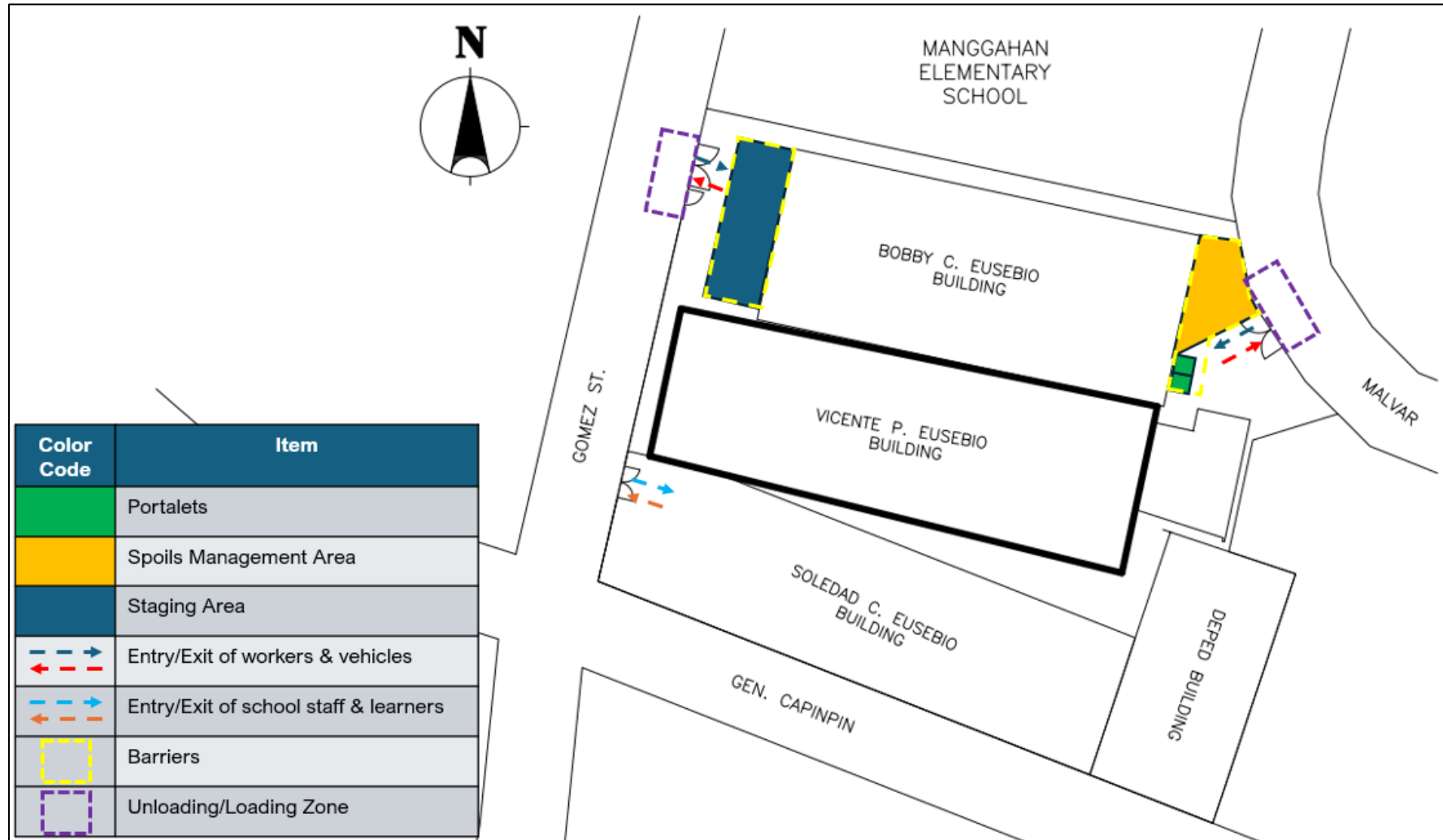
Figure 1-4: Proposed Staging Area and other Support Facilities in Manggahan Elementary School
