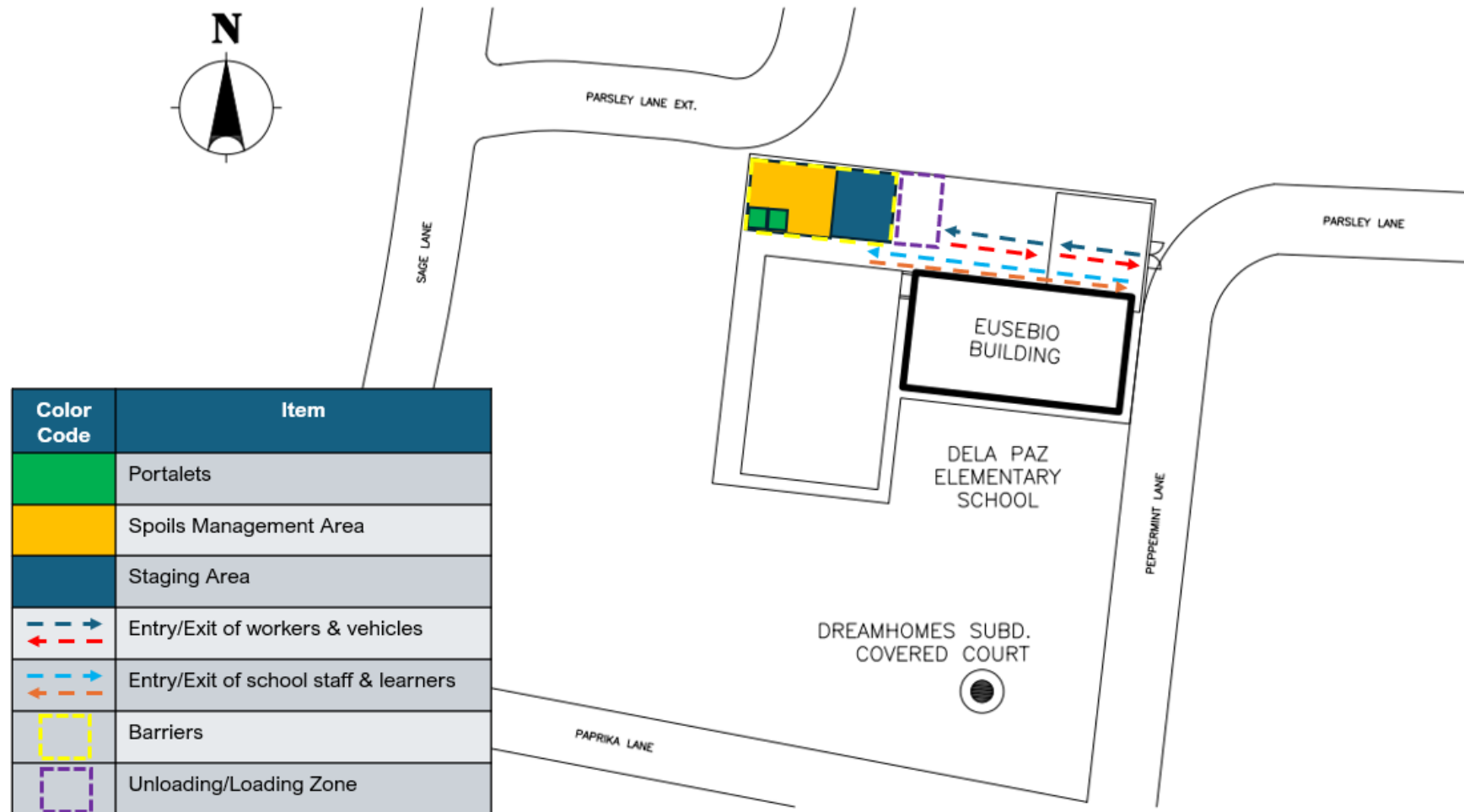
Figure 1-4: Proposed Staging Area and other Support Facilities in Dela Paz Elementary School
