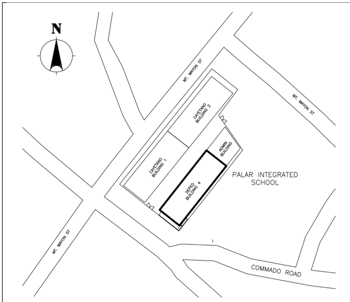
Figure 2-4: Site Development Plan of Palar Integrated School
