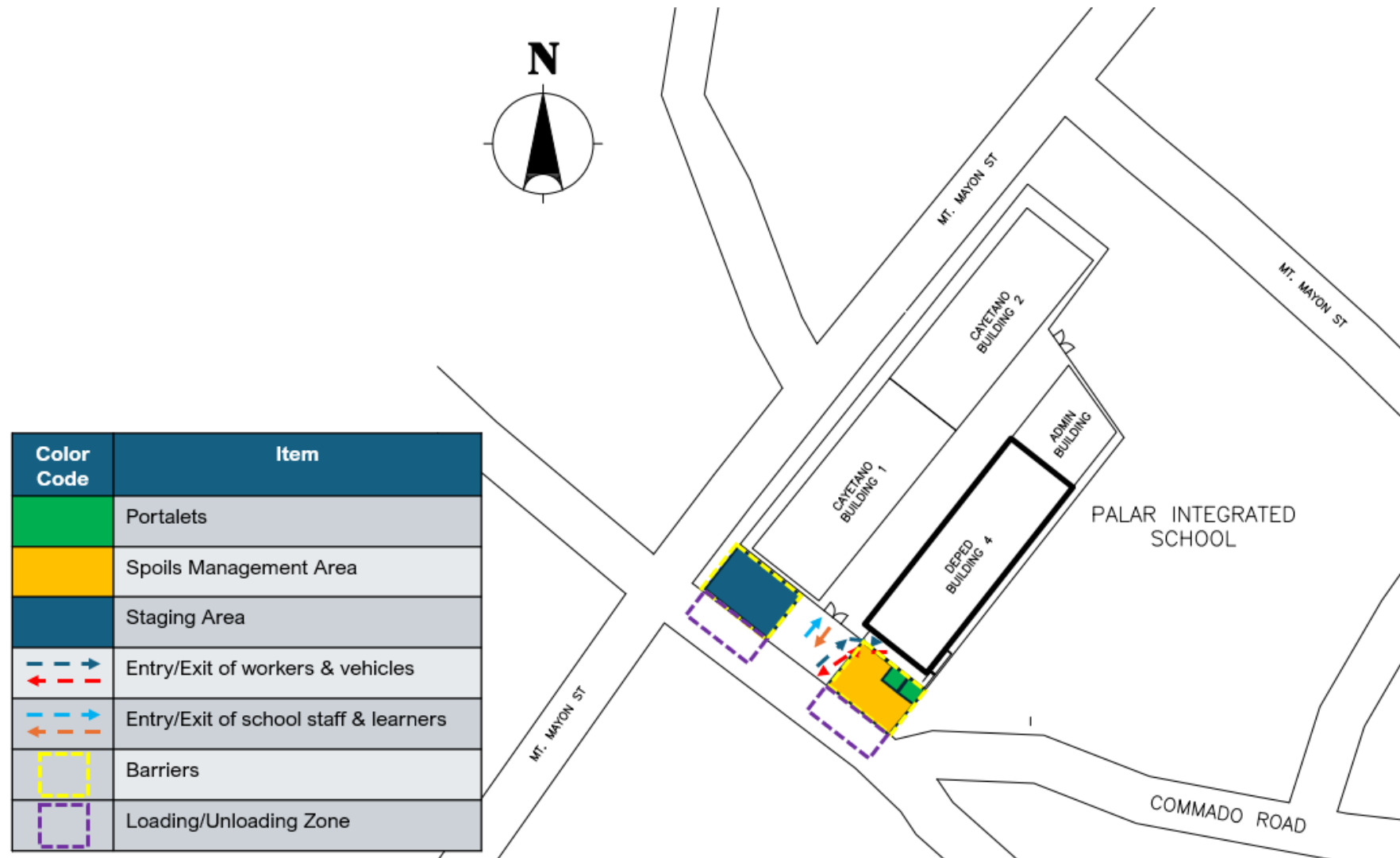
Figure 1-4: Proposed Staging Area and other Support Facilities in Palar Integrated School
