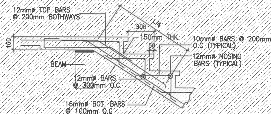
5 SPOT DETAIL D
