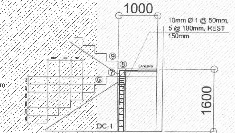
6 DETAIL SECTION DC-1
