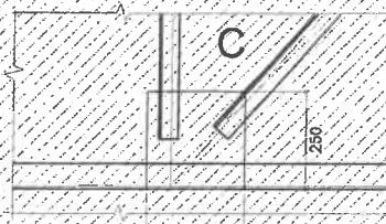
5 DETAIL-4 S-18 SCALE 1:10 M.
