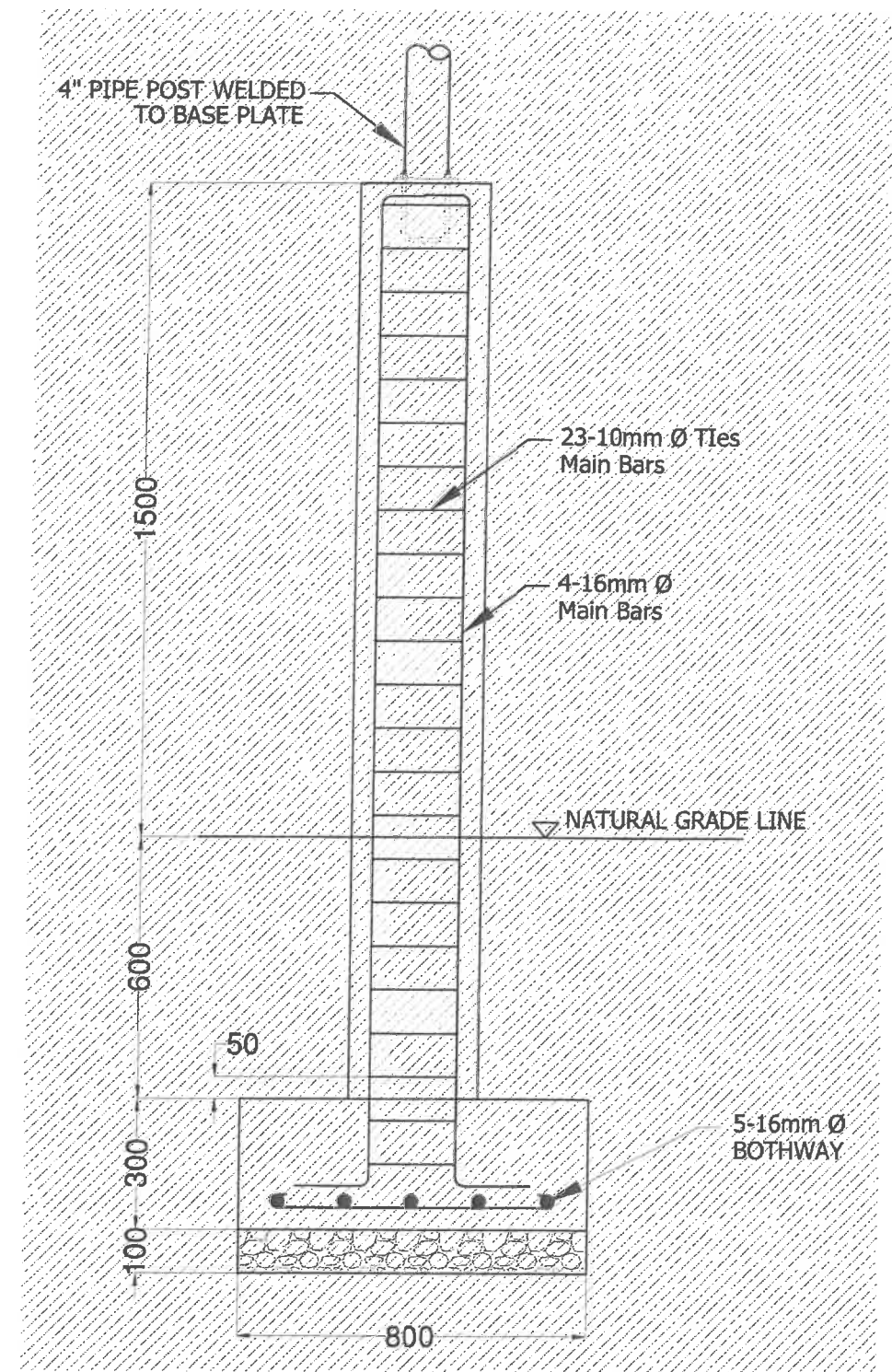
4 PEDESTAL COLUMN BAY SECTION DETAIL S-20 SCALE: NTS
