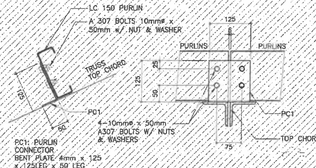
2A FOR NON - CONTINUOUS PURLINS S-18 SCALE 1:5 M.
