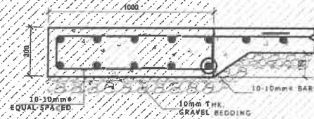
3 PEDESTAL COLUMN CONCRETE BASE SUPPORT S-20 SCALE: NTS
