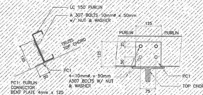
2B FOR CONTINUOUS PURLINS S-18 SCALE 1:5 M.
