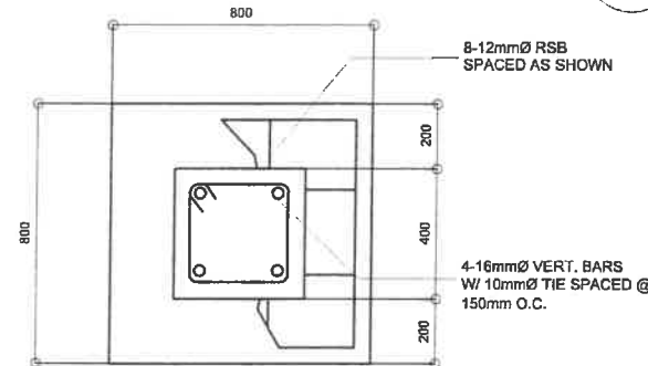
1 PEDESTAL COLUMN FOOTING PLAN DETAIL S-20 SCALE: NTS
