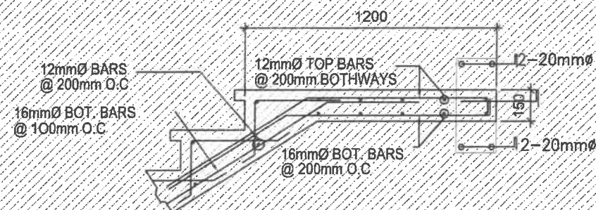
4 SPOT DETAIL C
