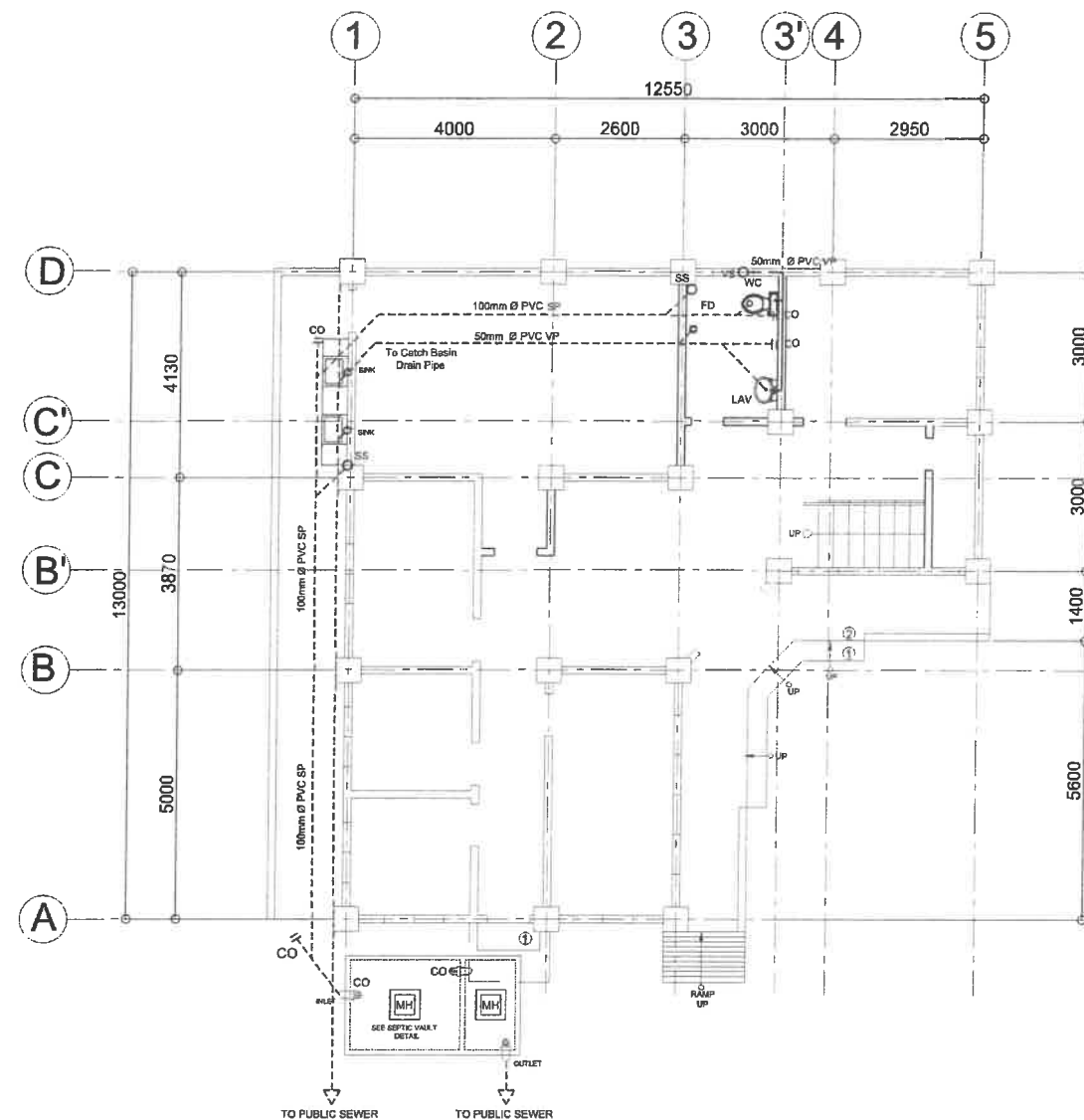
1 GROUND FLOOR SANITARY LAYOUT P-1 SCALE: 1:100M
