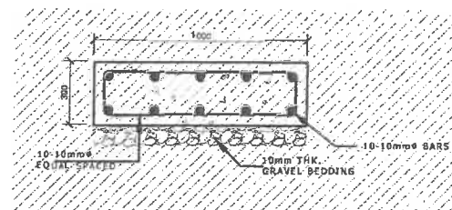
2 PEDESTAL COLUMN FOOTING DETAIL SECT. S-20 SCALE: NTS
