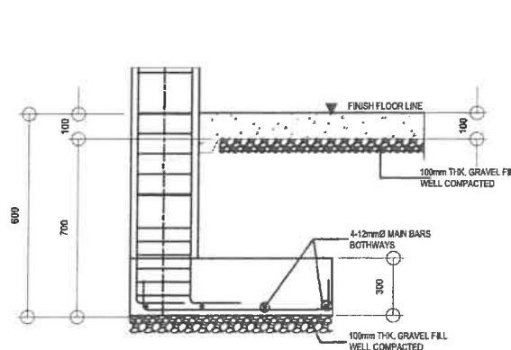
6 PERIMETER COLUMN DETAIL SECT. OF C4-F4 S-20 SCALE: 1:20 NTS
