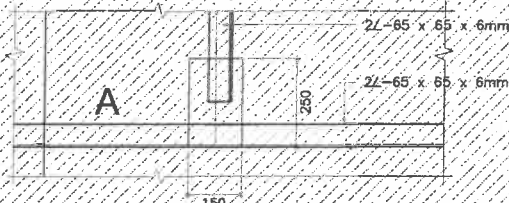
2 DETAIL S-18 SCALE 1:10 M.
