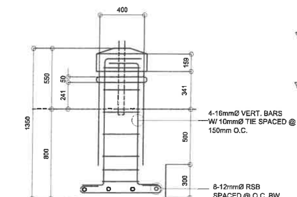
8 SPOT SECTION DET LAMP POST S-20 SCALE: 1:20 NTS
