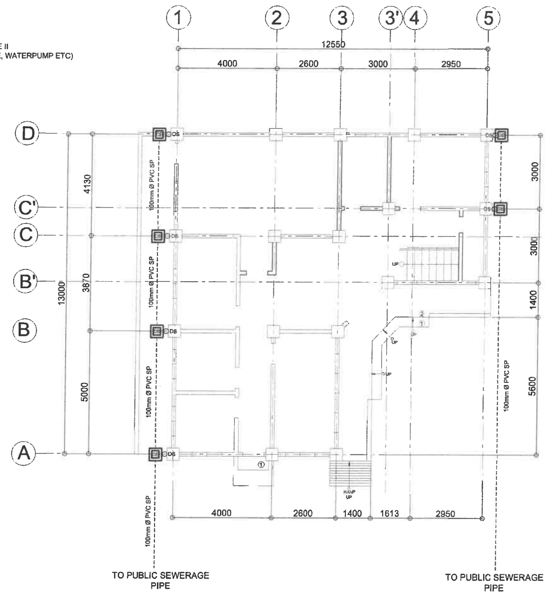
2 GROUND FLOOR STORM WATER LAYOUT P-4 SCALE: 1:100M
