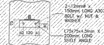
8B SECTION S-18 SCALE 1:10 M.
