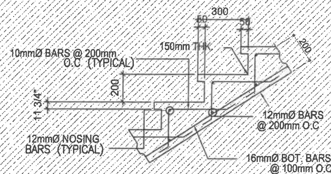
3 SPOT DETAIL B
