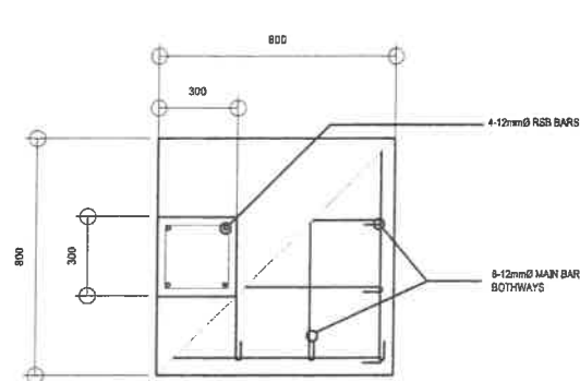
5 PERIMETER FOOTING DETAIL PLAN OF C4-F4 S-20 SCALE: 1:20 NTS
