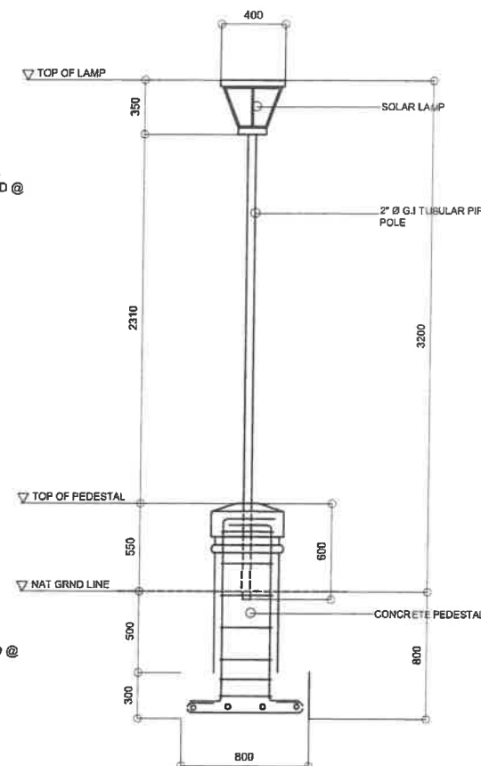
9 DETAIL SECTION LAMP POST S-20 SCALE: 1:30 NTS
