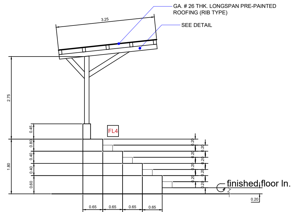
4 4-STEPS BLEACHER TYPICAL ELEVATION SCALE 1:50 MTRS.
