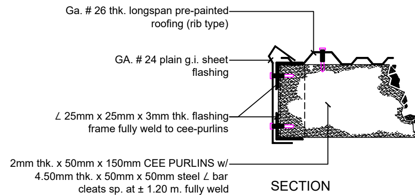
3 FLASHING DETAIL DRAWN NOT SCALED
