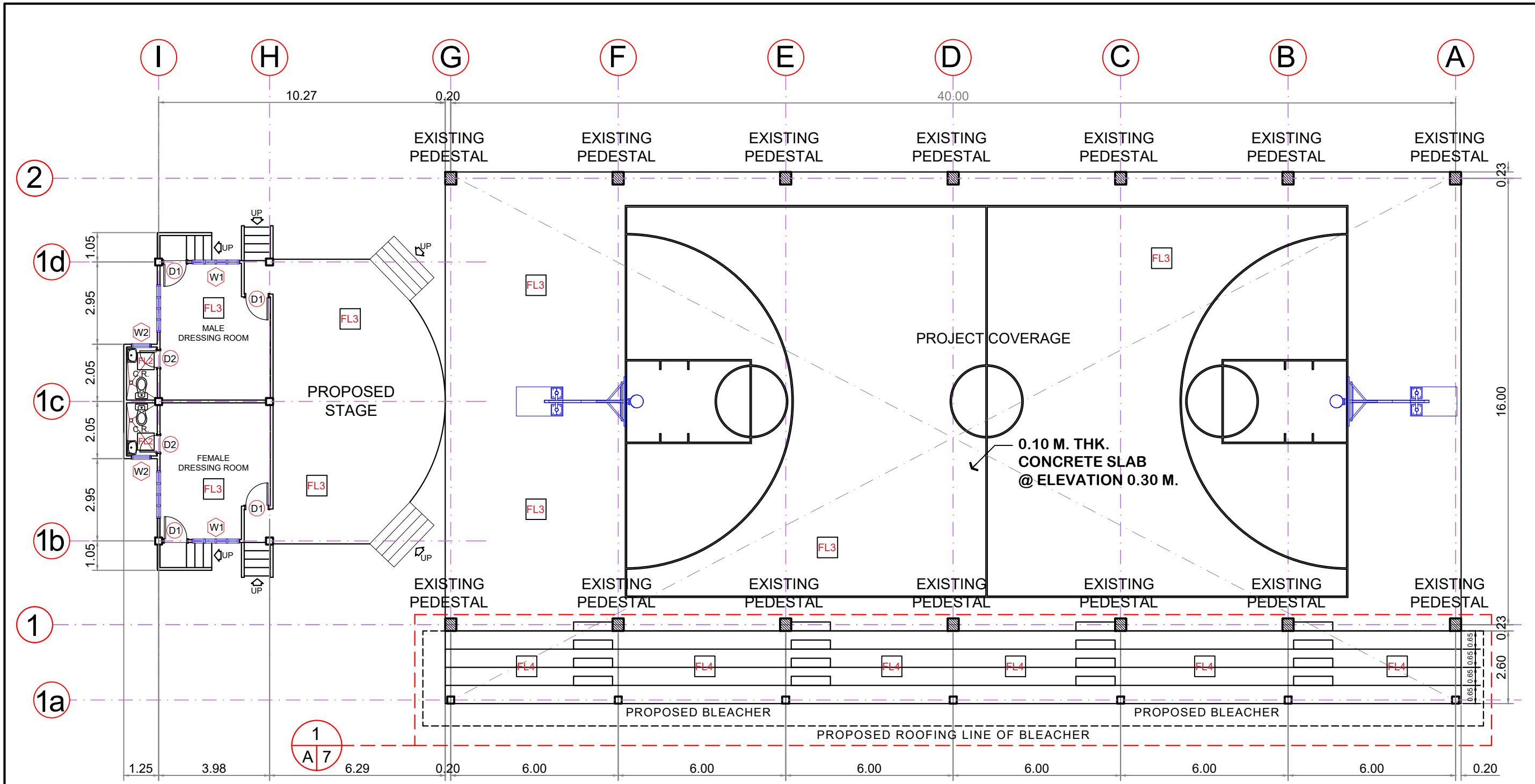
1 FLOOR PLAN SCALE 1:100 MTRS.
