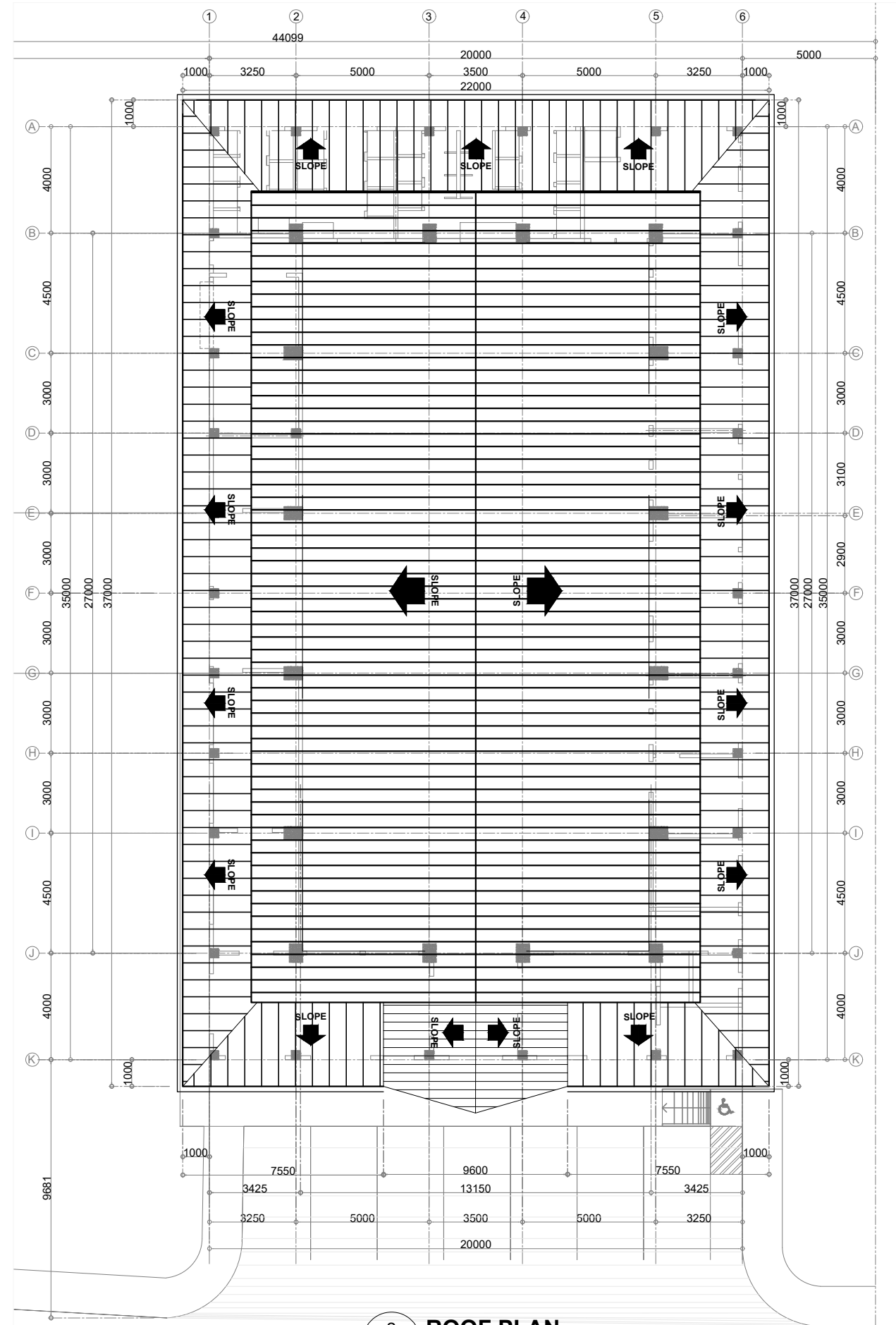
2 ROOF PLAN A 2 SCALE: 1:200M
