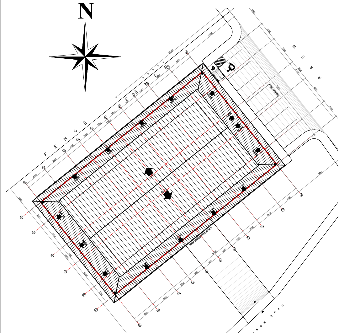
2 A 0 SITE DEVELOPMENT PLAN SCALE: 1:400 M
