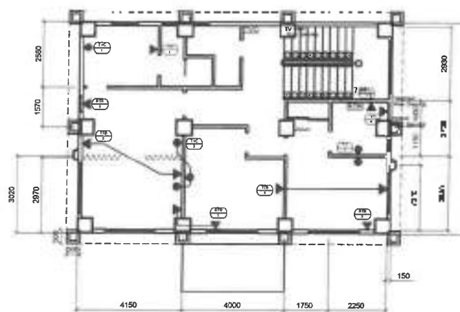
4 SECOND FLOOR TELECOMMUNICATION LAYOUT E-5 SCALE 1:100
