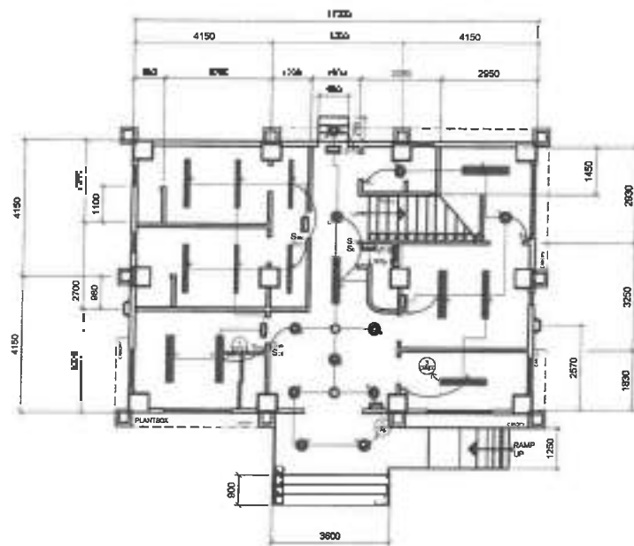
1 GROUND FLOOR LIGHTING LAYOUT E-4 SCALE 1:100
