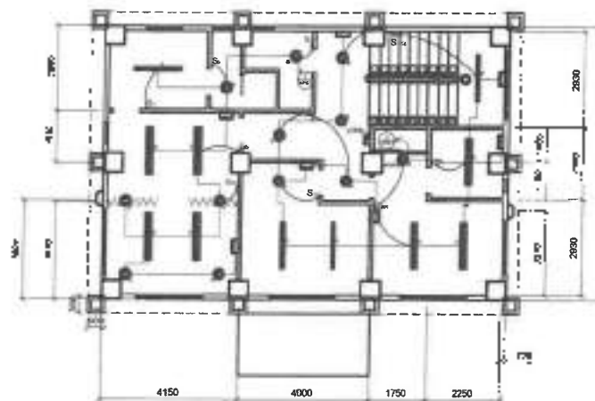
2 SECOND FLOOR LIGHTING LAYOUT E-4 SCALE 1:100
