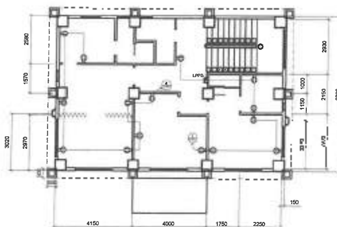
5 SECOND FLOOR POWER LAYOUT E-4 SCALE 1:100
