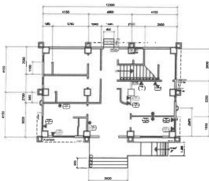
3 GROUND FLOOR TELECOMMUNICATION LAYOUT E-5 SCALE 1:100
