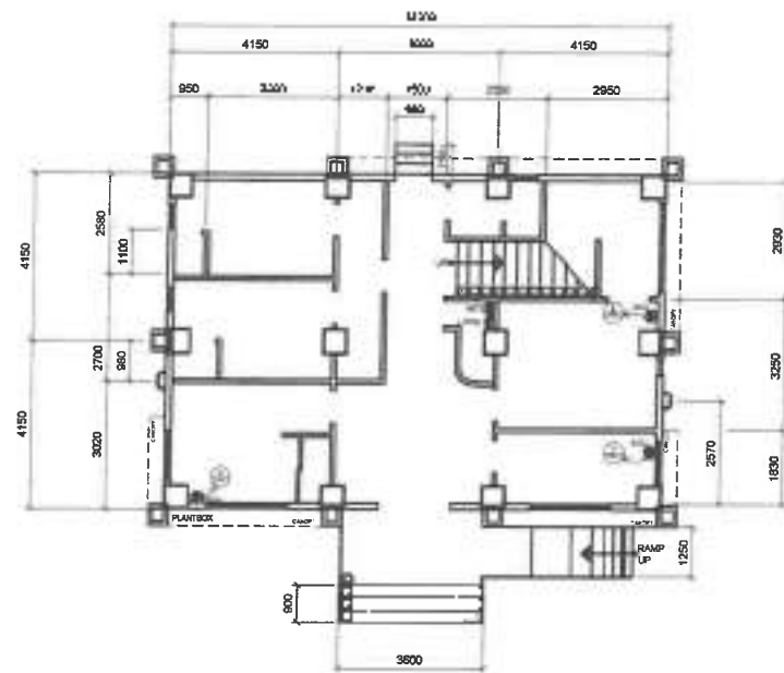
1 GROUND FLOOR ACU LAYOUT E-5 SCALE 1:100
