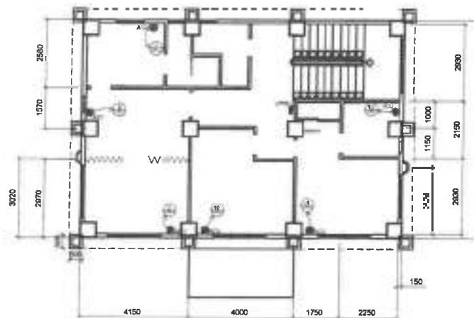
2 SECOND FLOOR ACU LAYOUT E-5 SCALE 1:100
