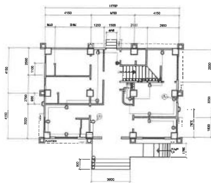
4 GROUND FLOOR POWER LAYOUT E-4 SCALE 1:100
