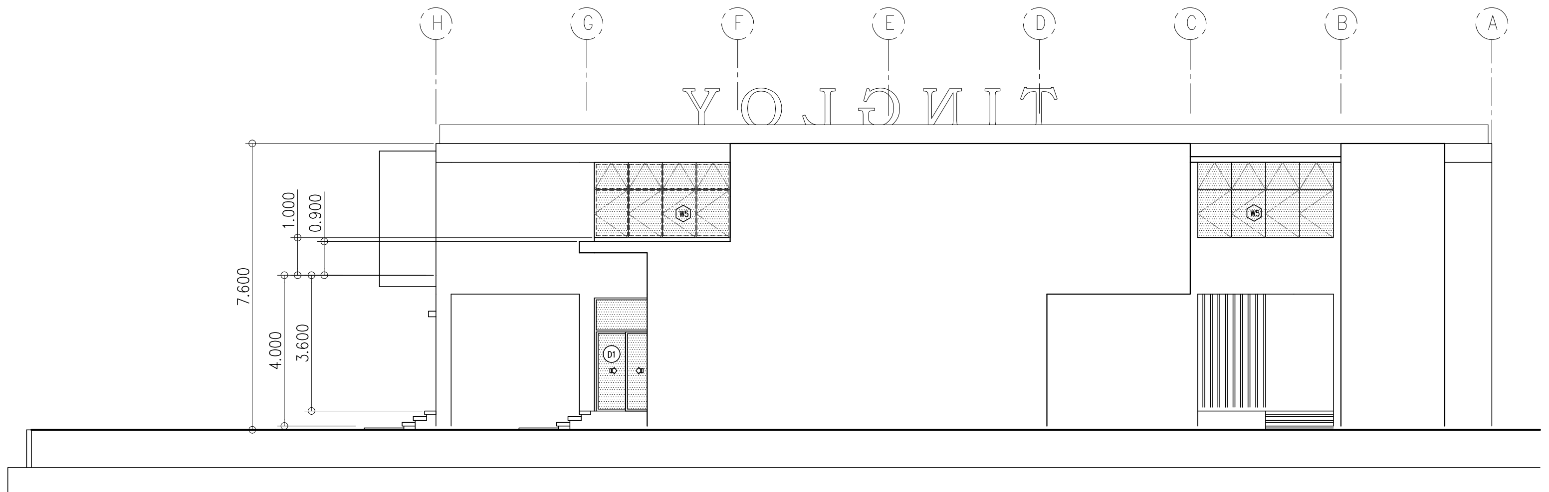
2 LEFT-SIDE ELEVATION A-3 SCALE 1:100 MTS.
