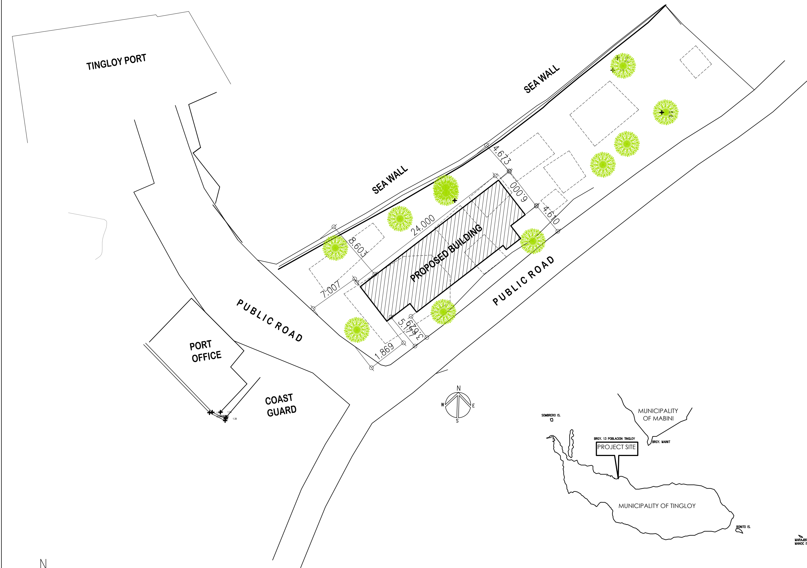
GROSS AREA = 385.52 SQ. M. SITE DEVELOPMENT PLAN 1 : 300 MTS.
