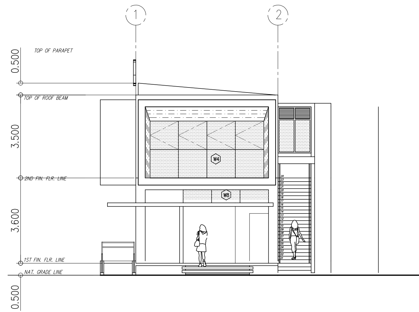
1 FRONT ELEVATION A-3 SCALE 1:100 MTS.
