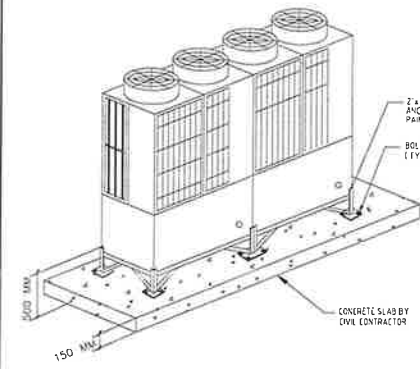
1 VRF MOUNTING DETAIL M-08 SCALE NTS
