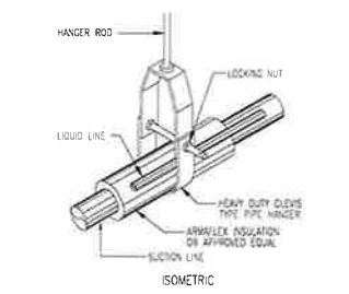
8 PIPE SUPPORT DETAIL M-08 SCALE NTS
