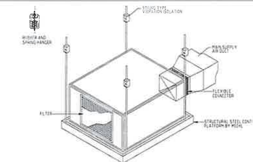
9 CEILING CONCEALED ACU MOUNTING DETAIL M-08 SCALE NTS
