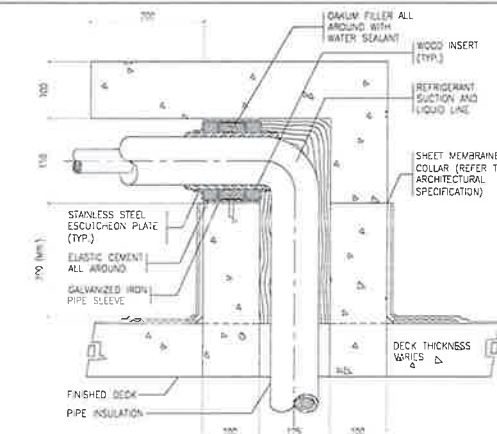
6 PIPE PENETRATION THRU ROOF DETAIL M-08 SCALE NTS
