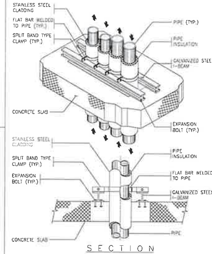
11 PIPE RISER SUPPORT DETAIL M-08 SCALE NTS
