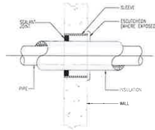
5 PIPE SLEEVE DETAIL M-08 SCALE NTS
