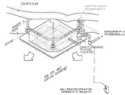
2 CEILING CASSETTE ACU MOUNTING DETAIL M-08 SCALE NTS
