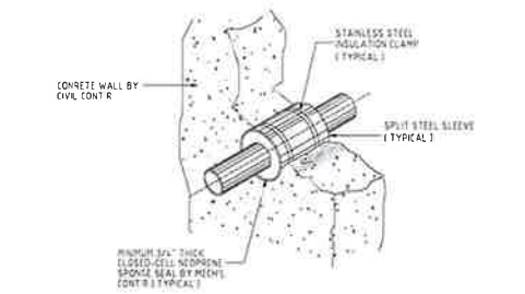
10 PIPE PENETRATION THRU WALL DETAIL M-08 SCALE NTS
