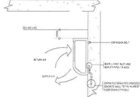
3 WALL MOUNTED ACU MOUNTING DETAIL M-08 SCALE NTS
