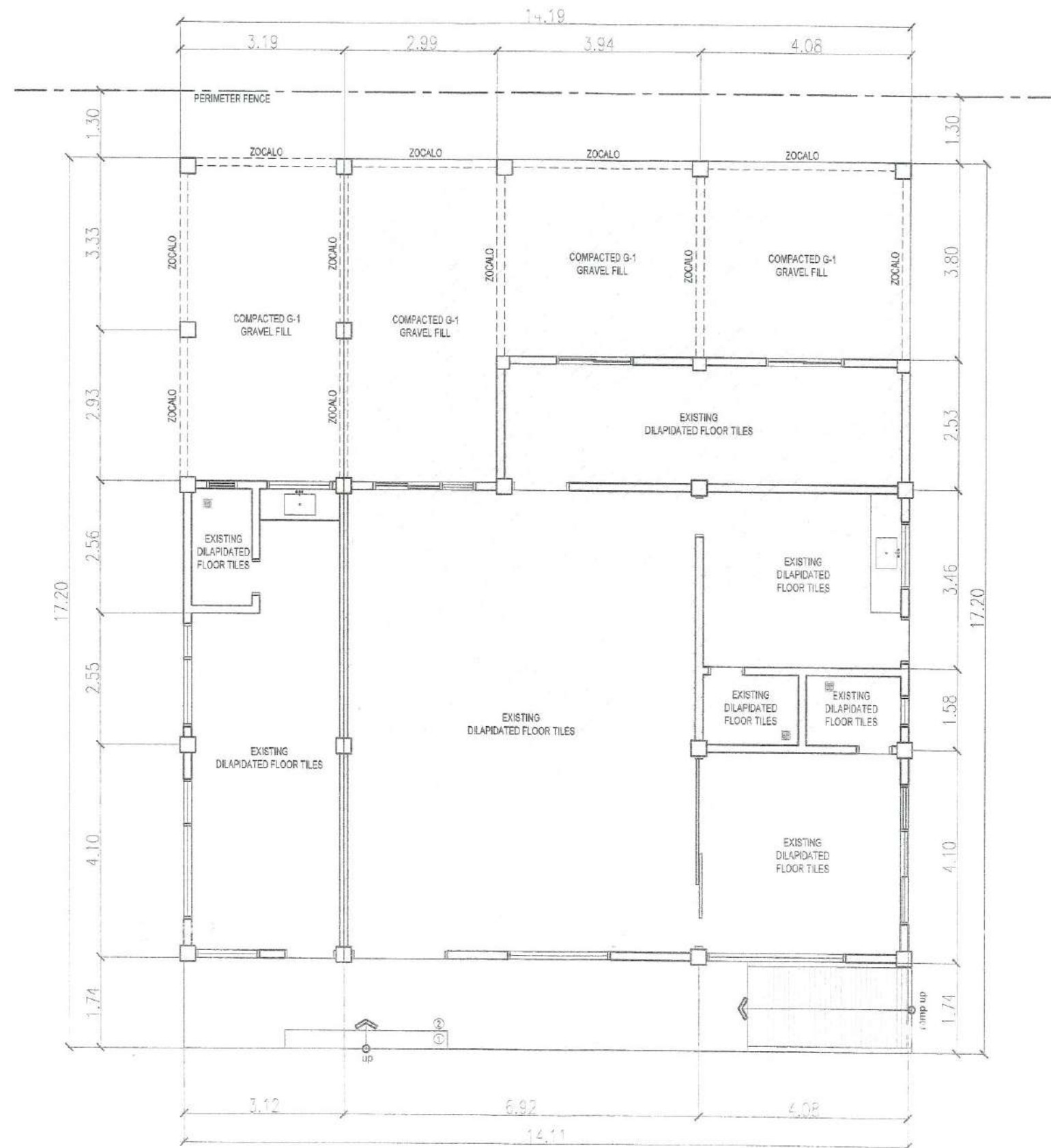
1 EXISTING FLOOR FINISH PLAN A - 3 SCALE: 1:100 MTS.
