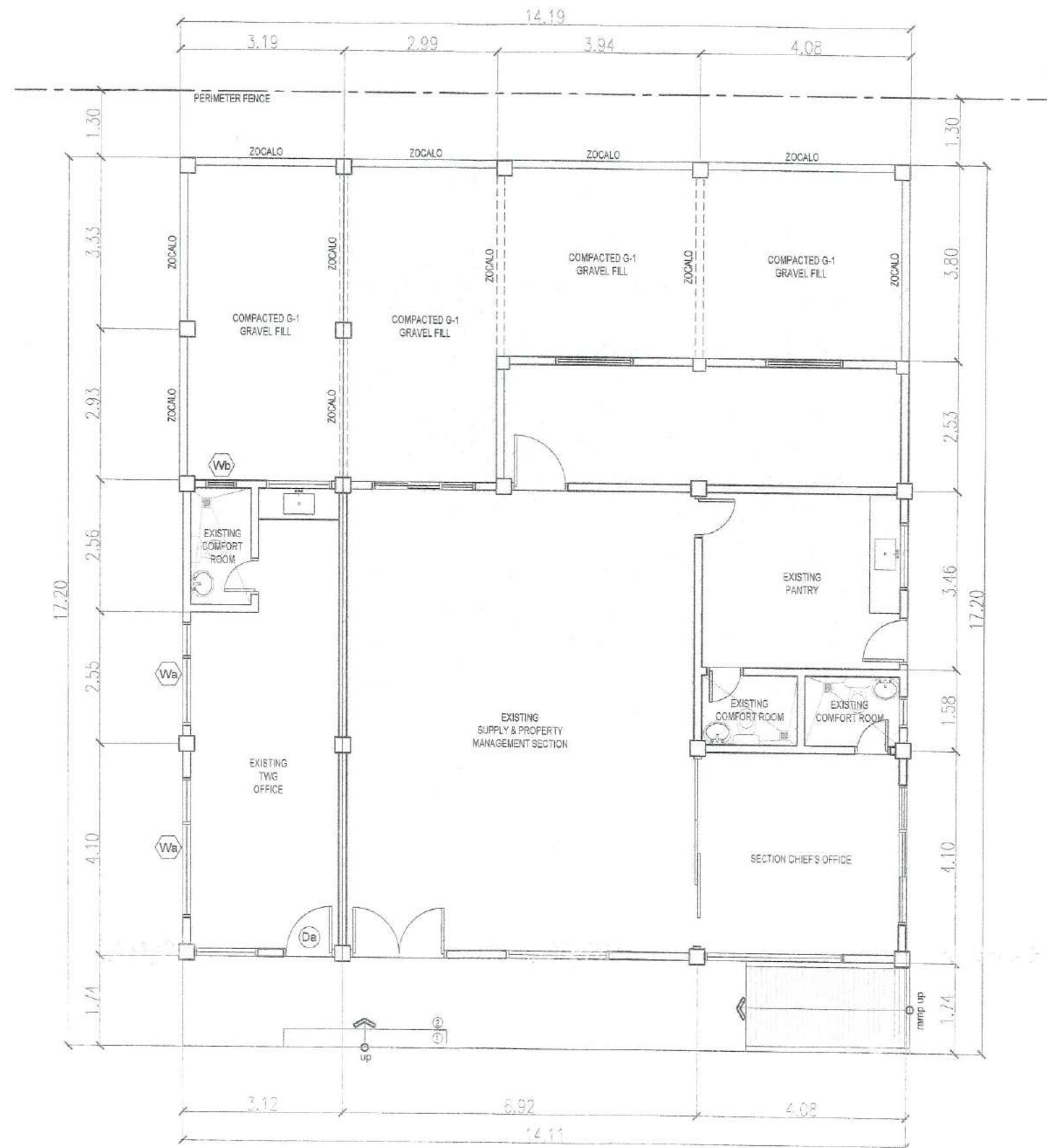
1 EXISTING GROUND FLOOR PLAN A - 1 SCALE: 1:100 MTS.
