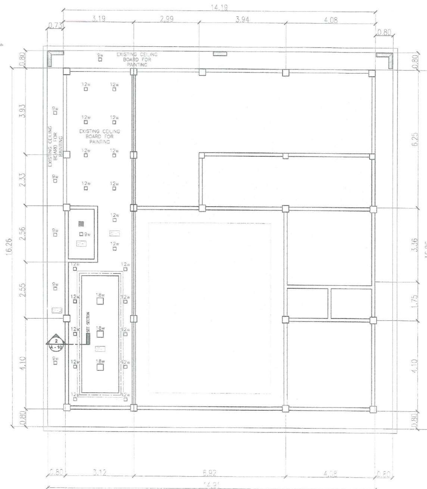
1 PROPOSED REFLECTED CEILING PLAN A - 6 SCALE: 1:100 MTS.
