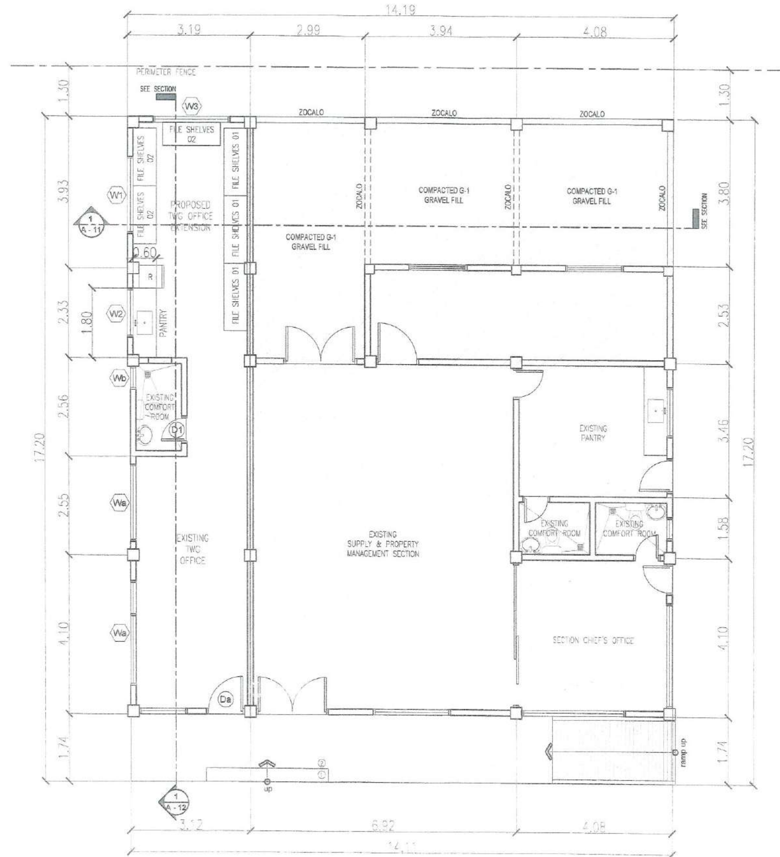
1 PROPOSED GROUND FLOOR PLAN A - 2 SCALE: 1:100 MTS.
